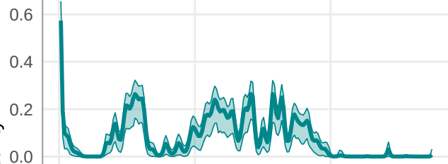
Cluster 5
