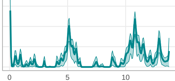
Cluster 3
