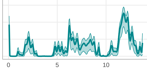
Cluster 4
