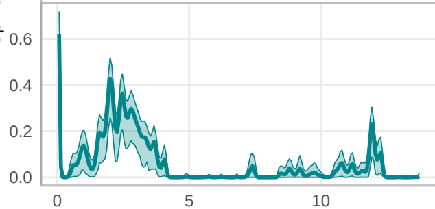
Cluster 5
