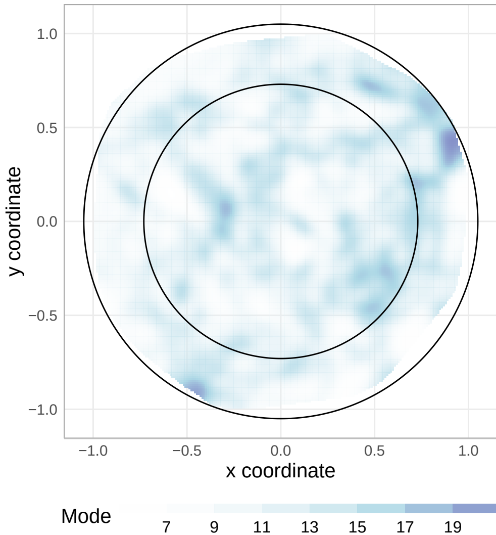
Posterior mode of the number of clusters
