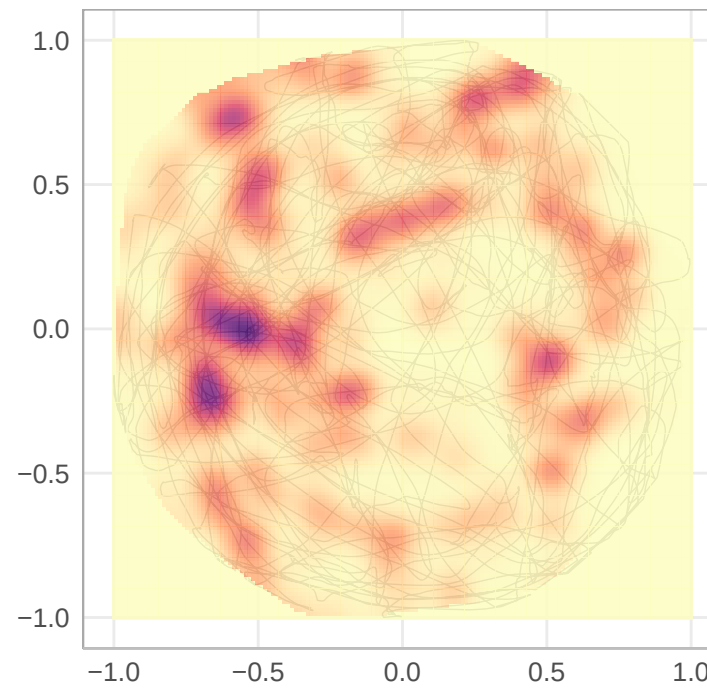
Neuron B
