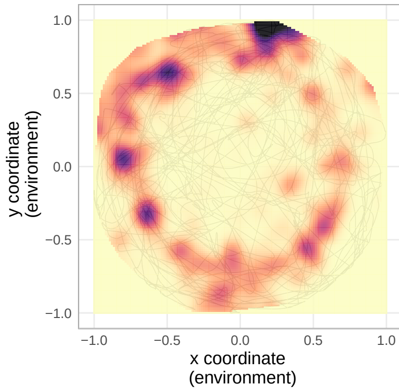
Neuron C
