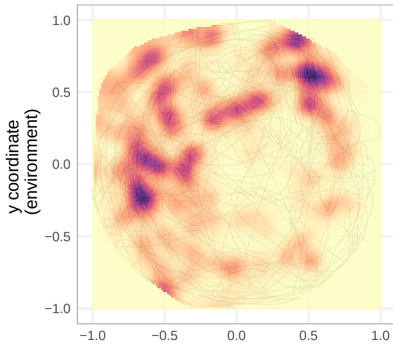
Neuron A
