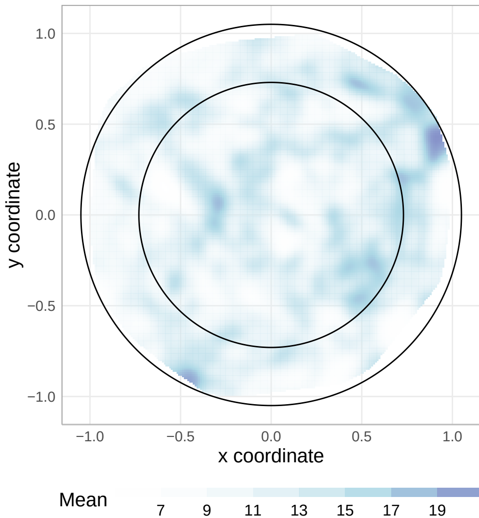
Posterior mean of the number of clusters
