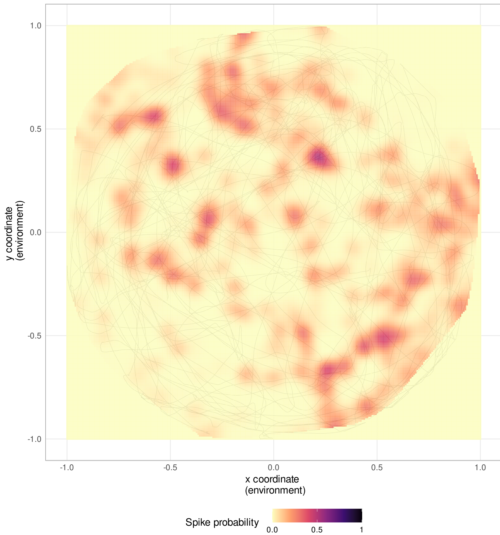
Neuron 106
