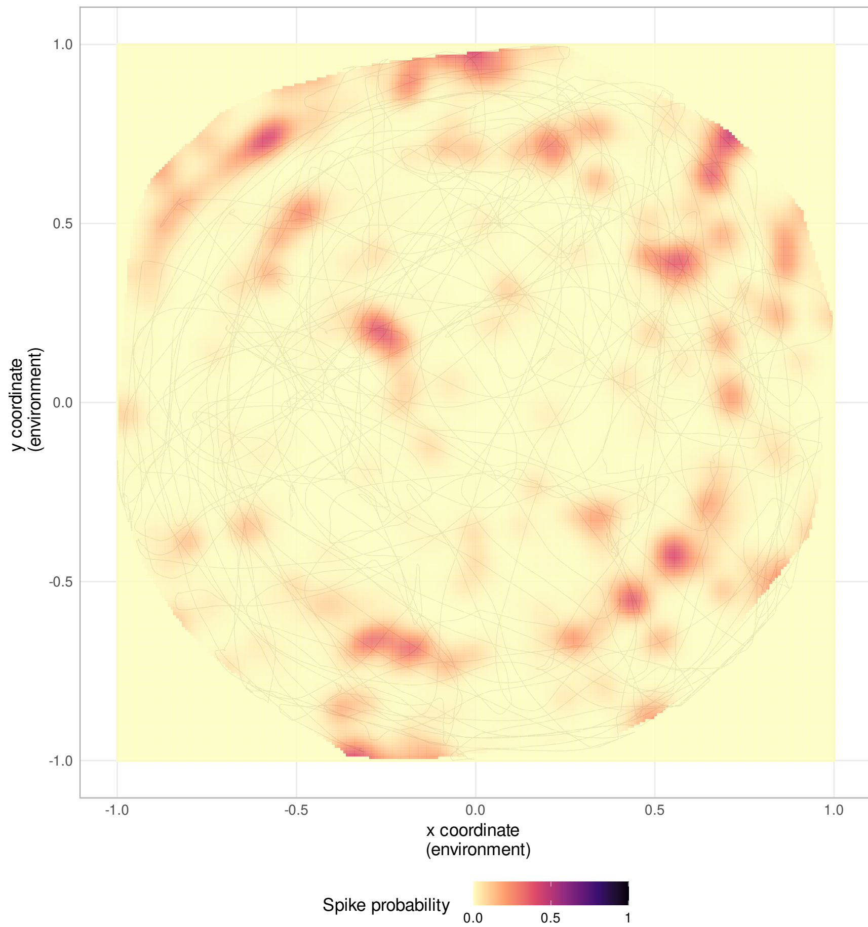
Neuron 109
