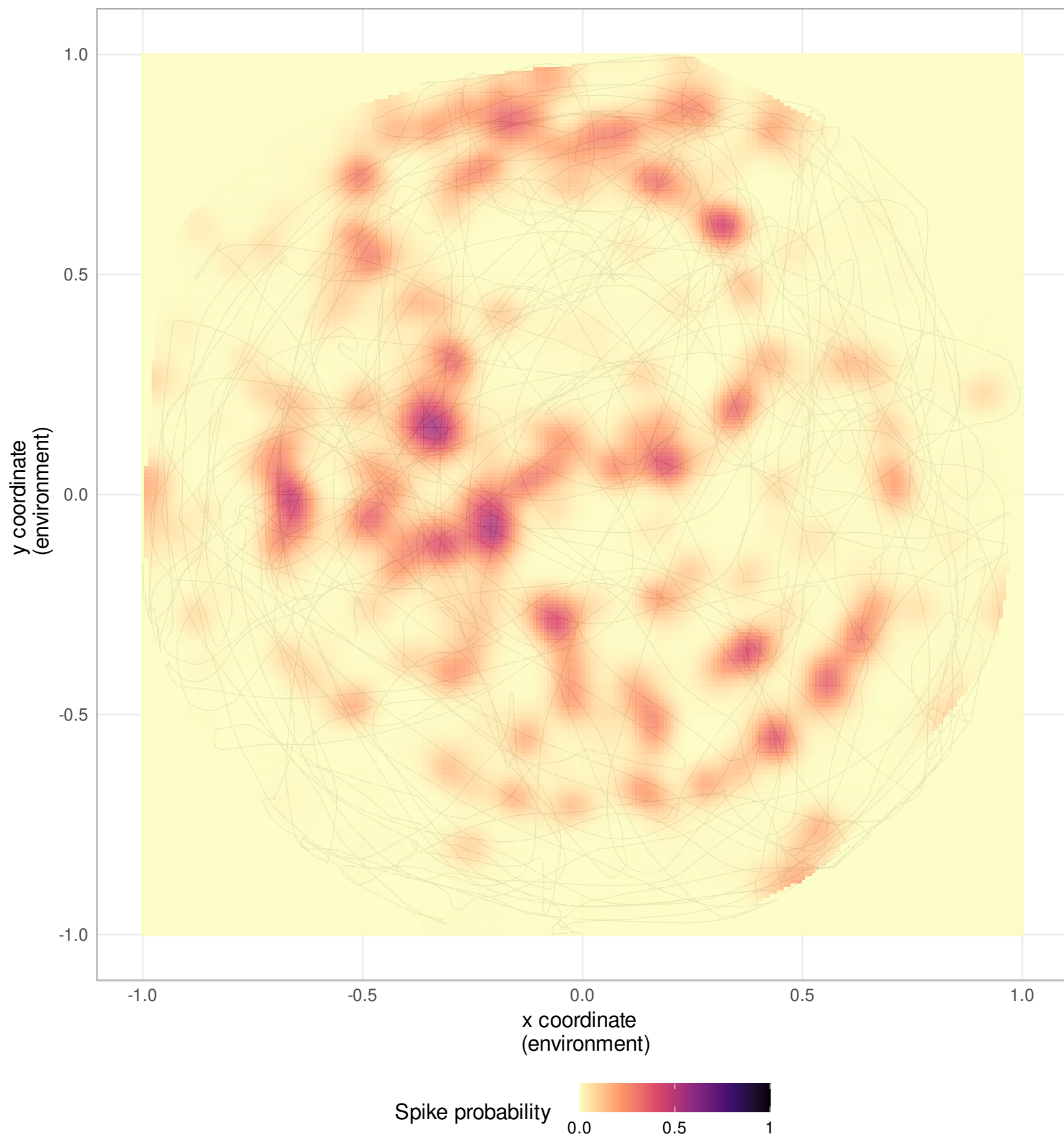
Neuron 111
