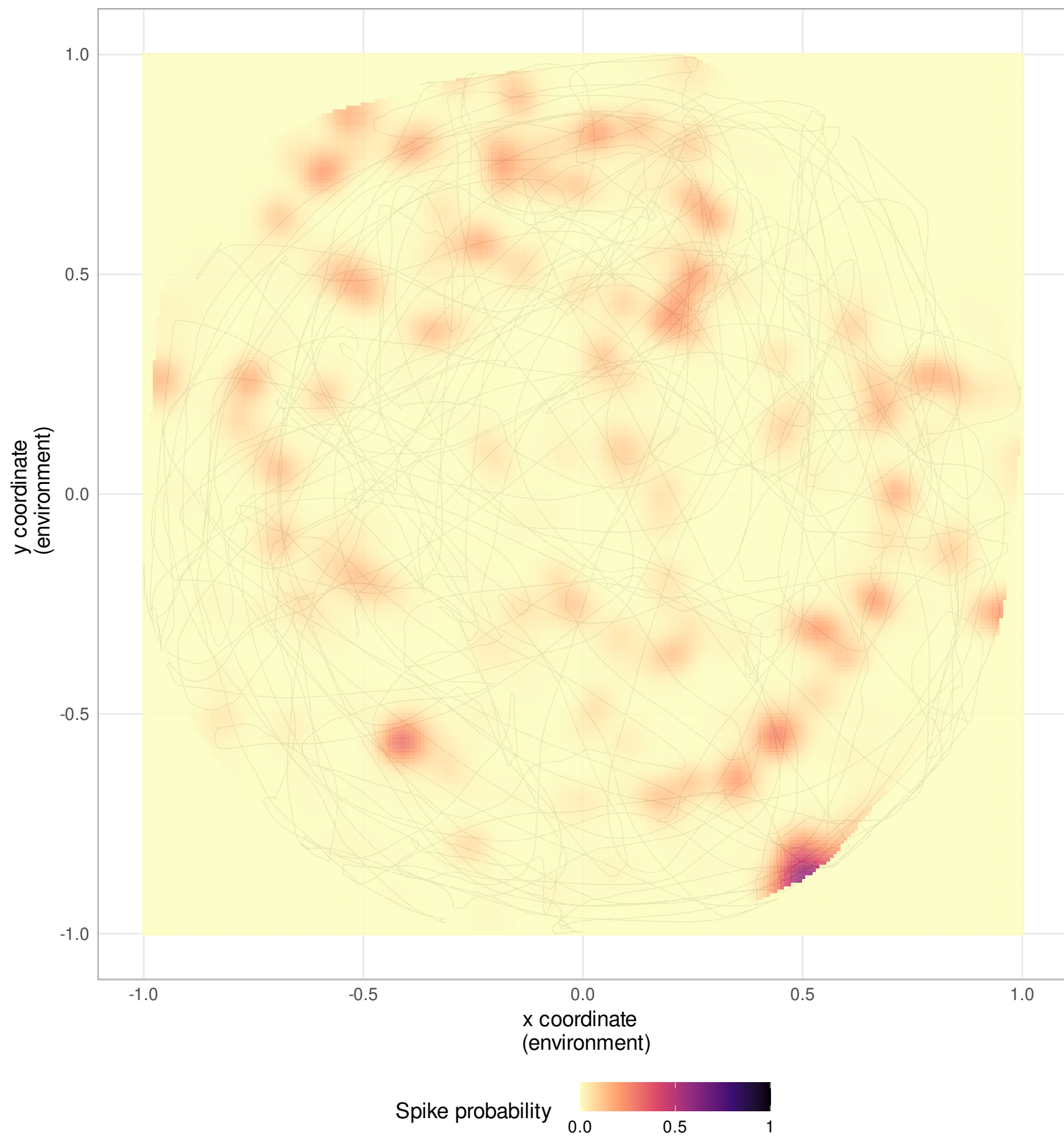
Neuron 112
