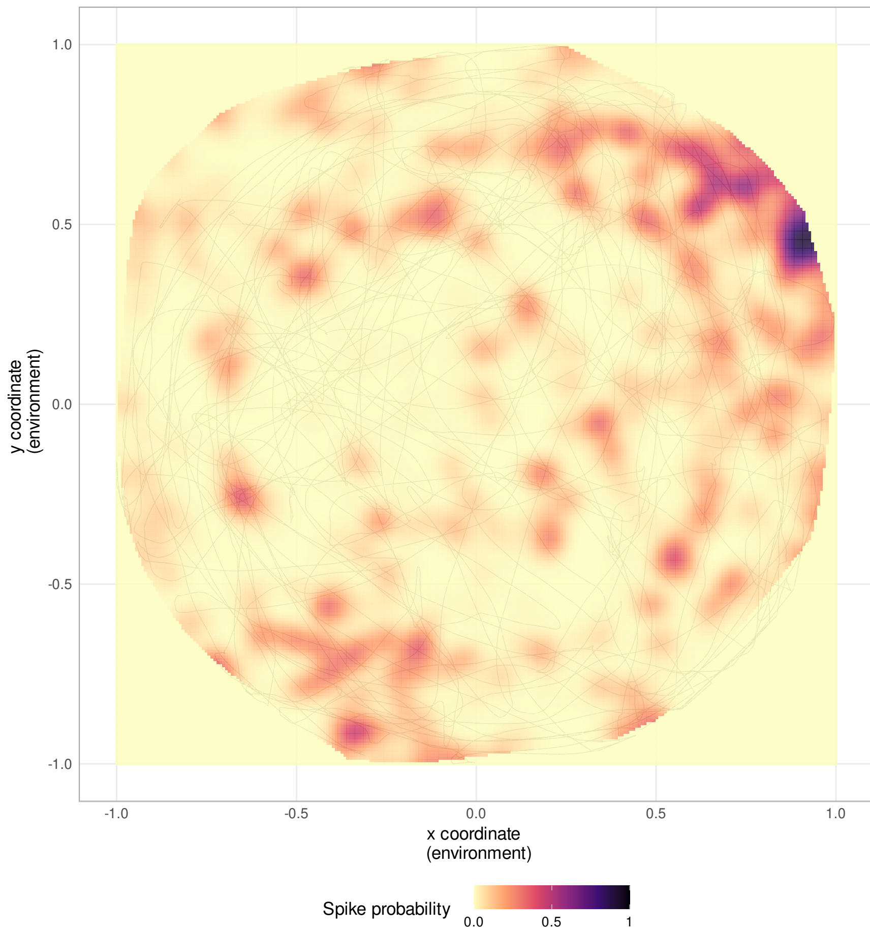
Neuron 115
