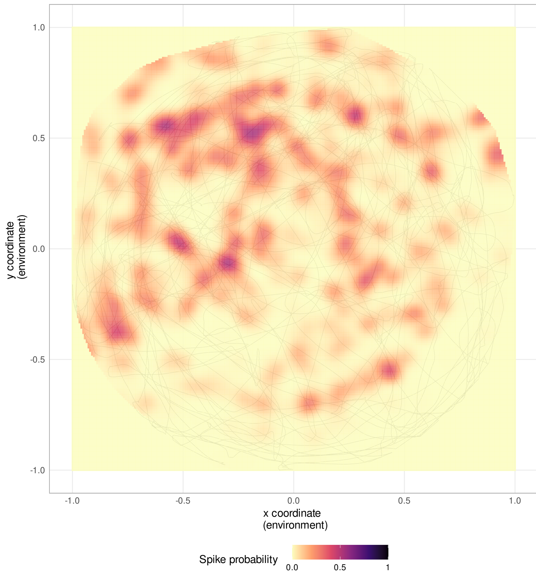
Neuron 116
