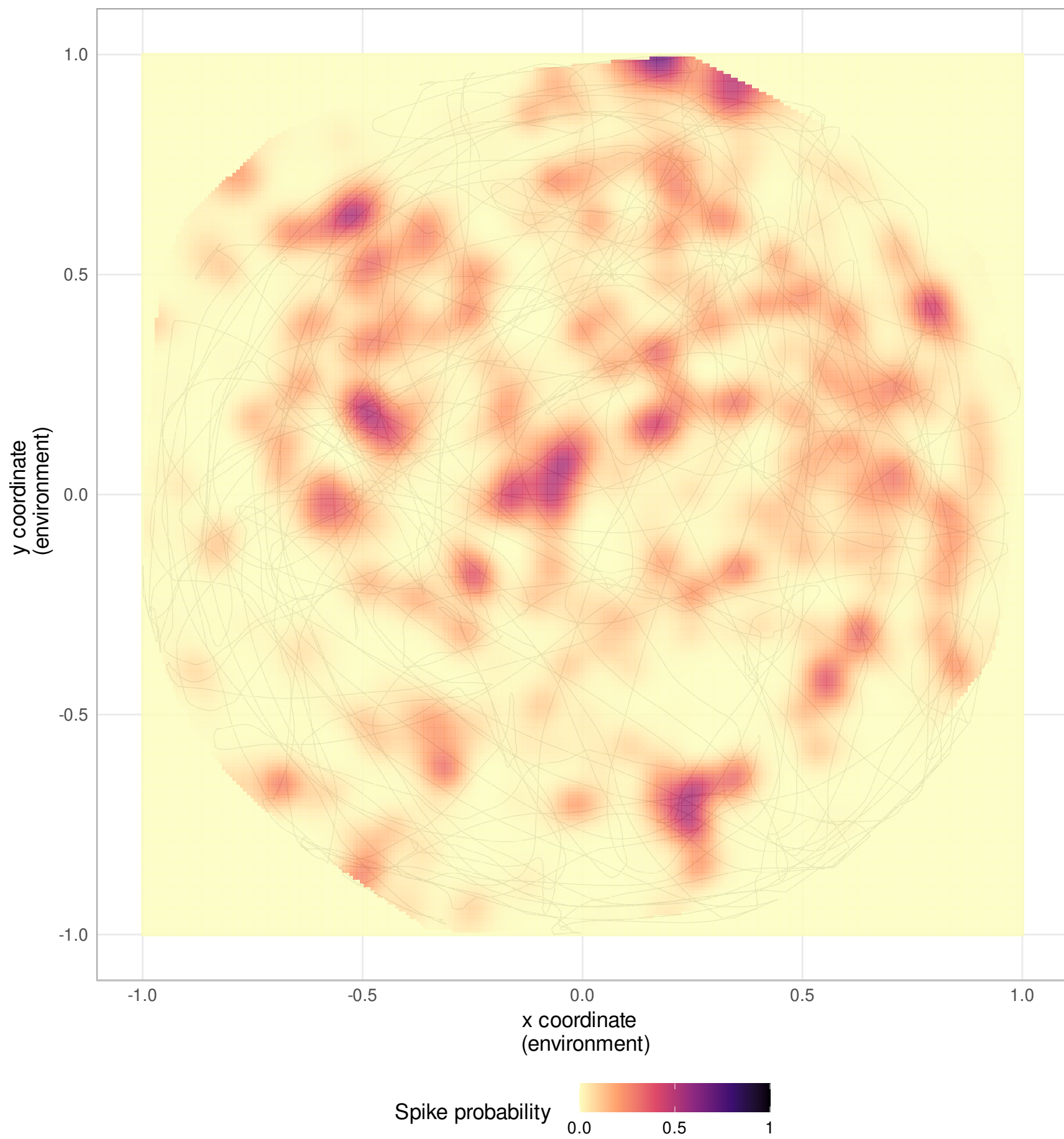
Neuron 123
