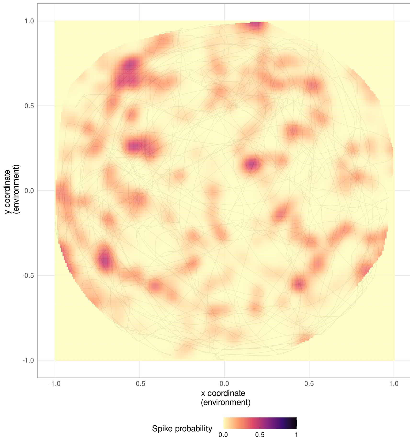
Neuron 127
