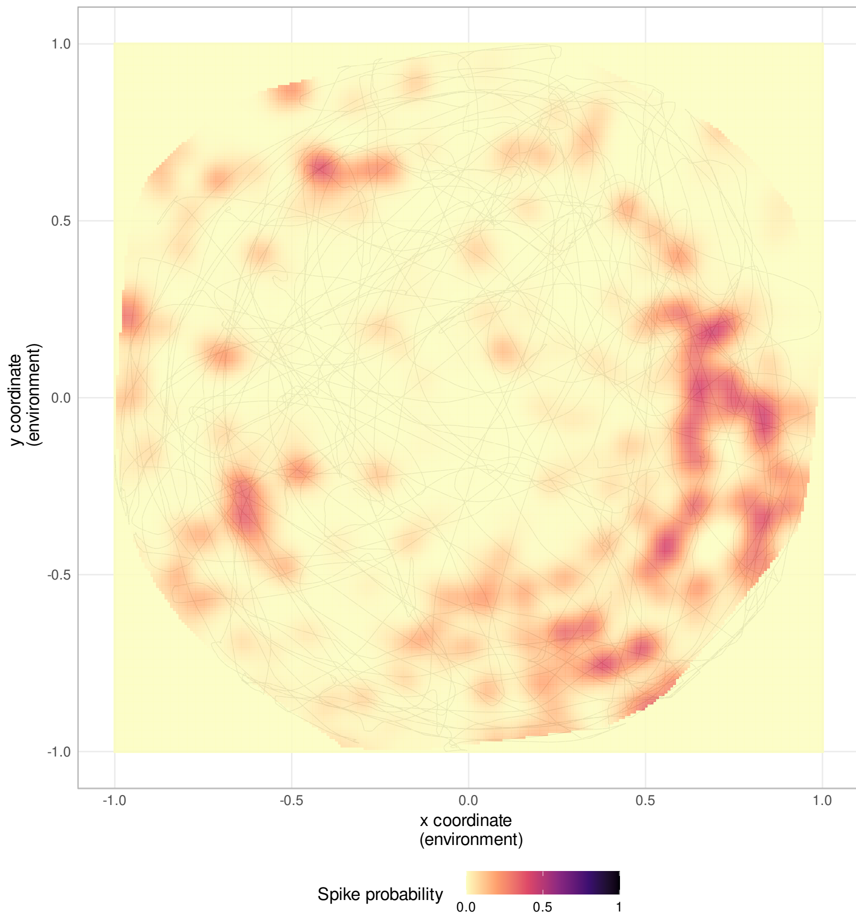
Neuron 128
