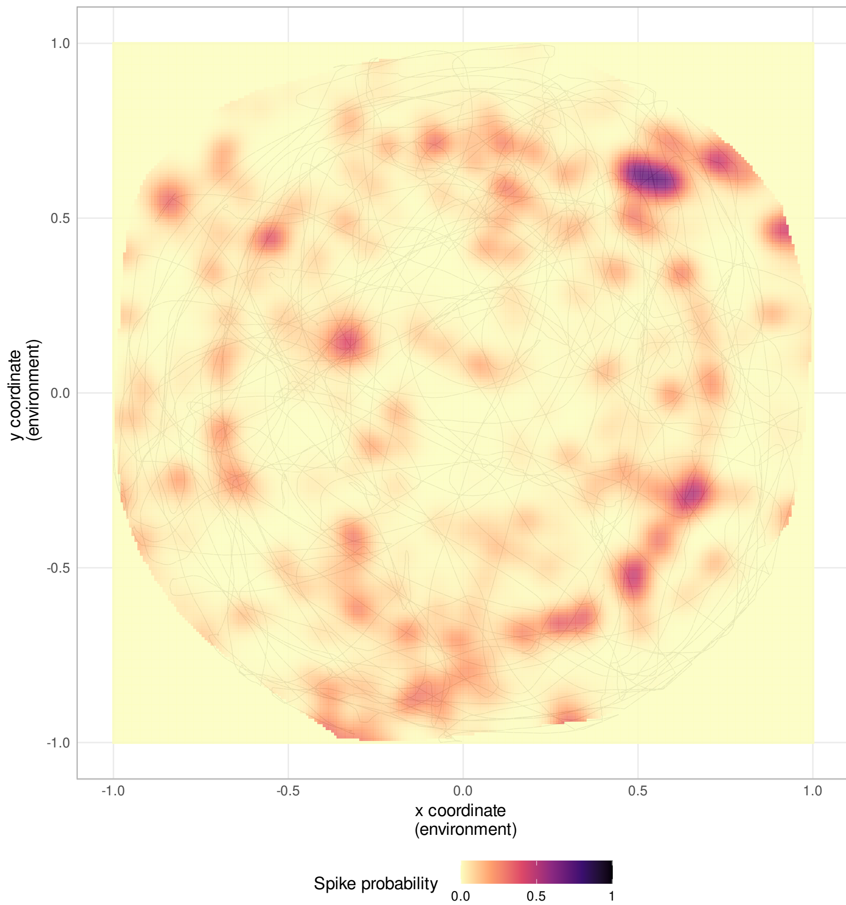
Neuron 13
