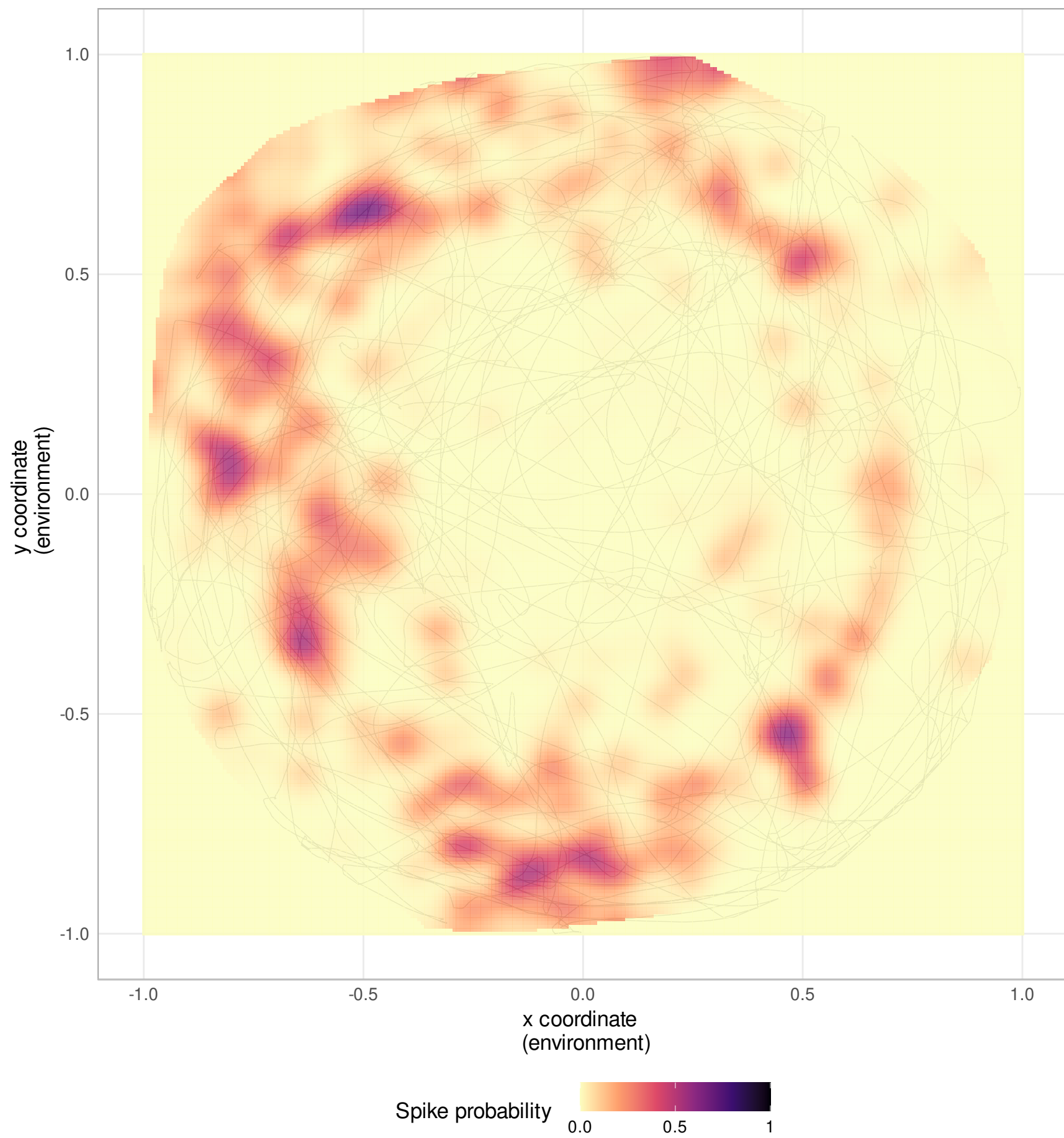
Neuron 130
