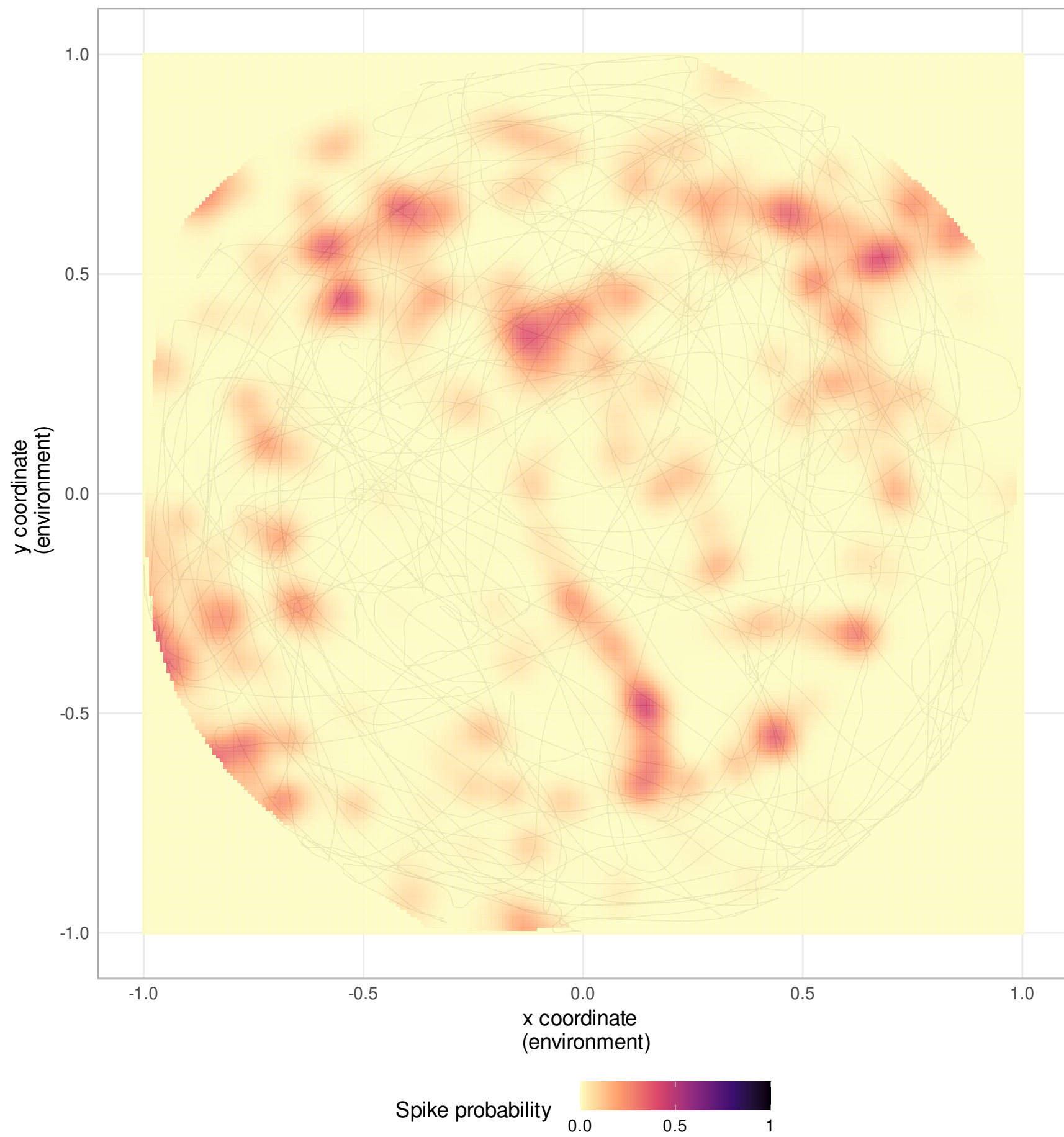
Neuron 132
