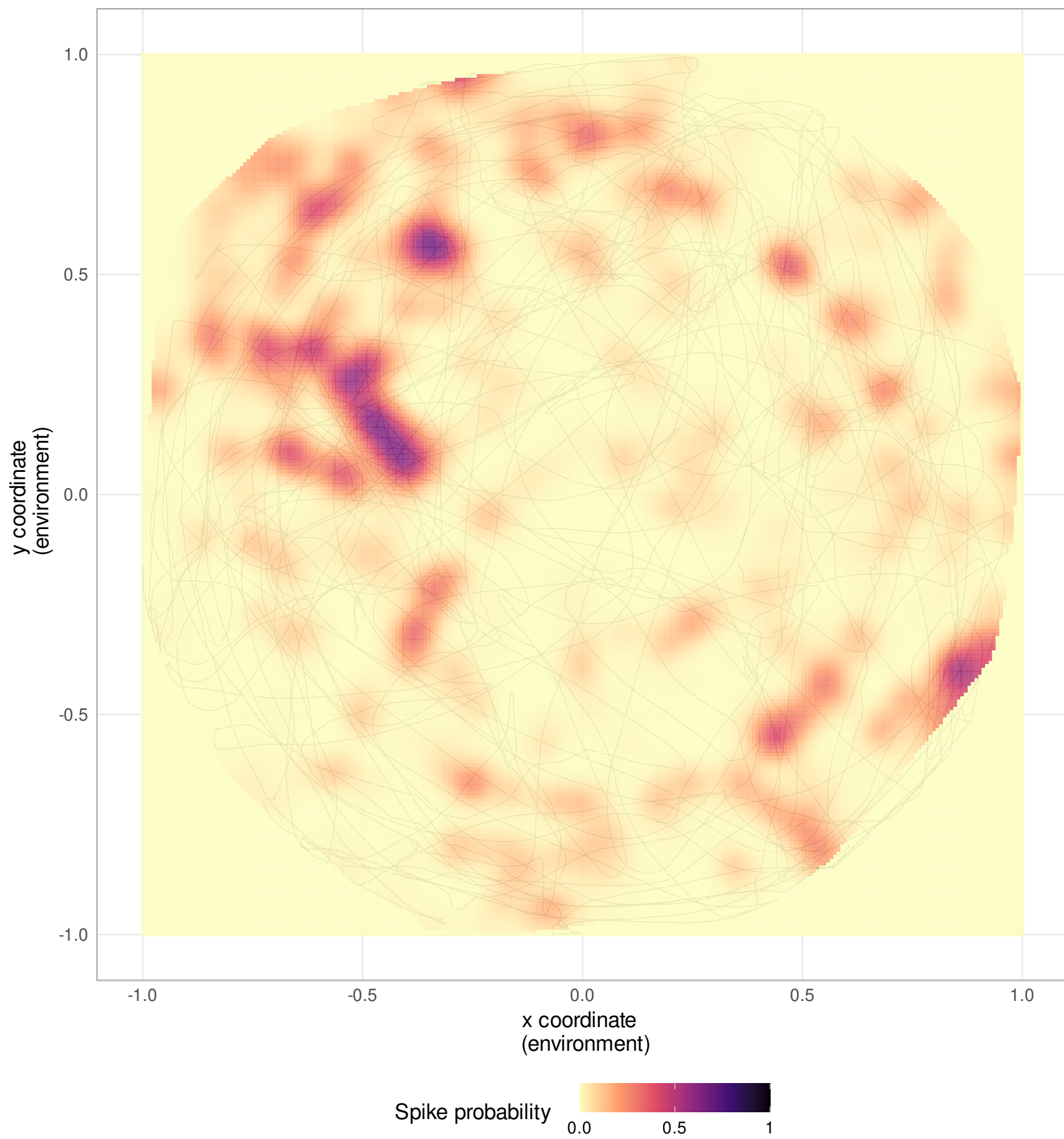
Neuron 136
