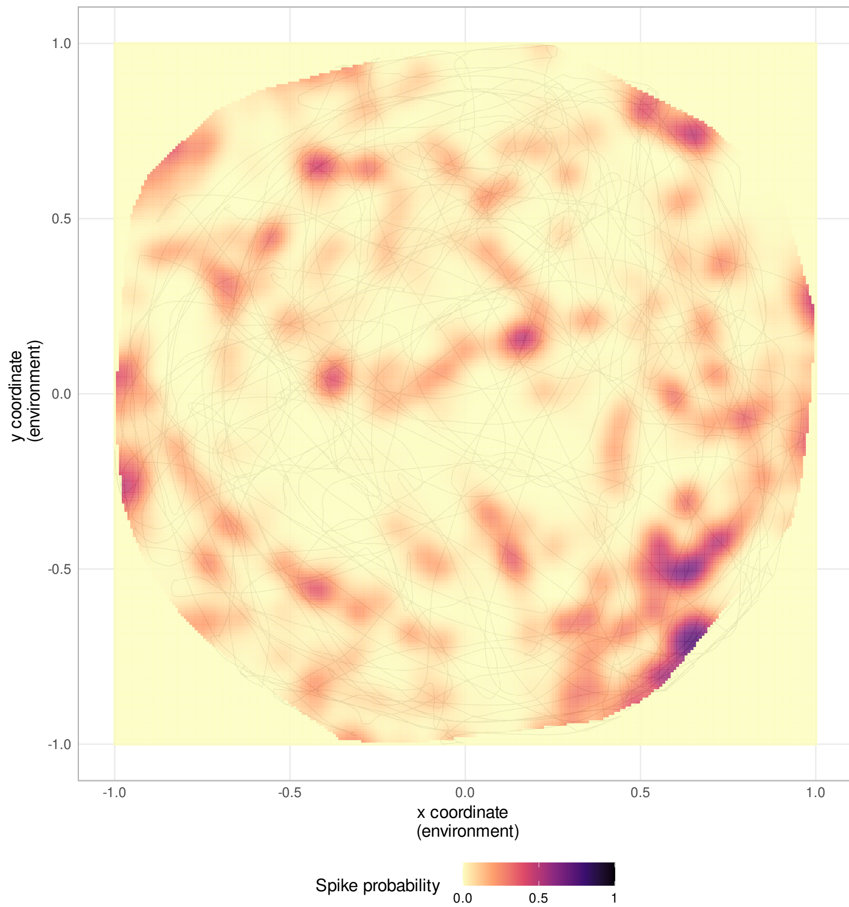
Neuron 138
