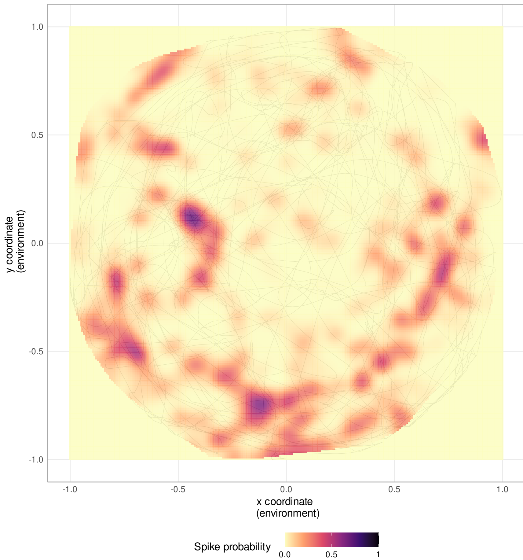
Neuron 16
