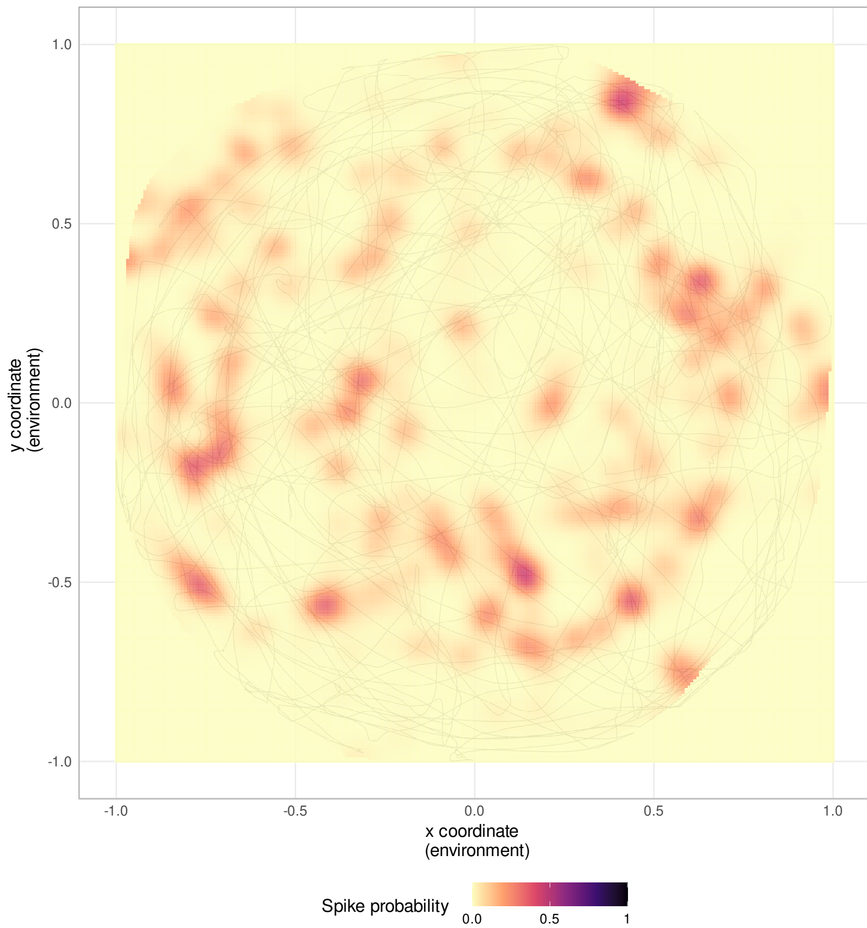
Neuron 164
