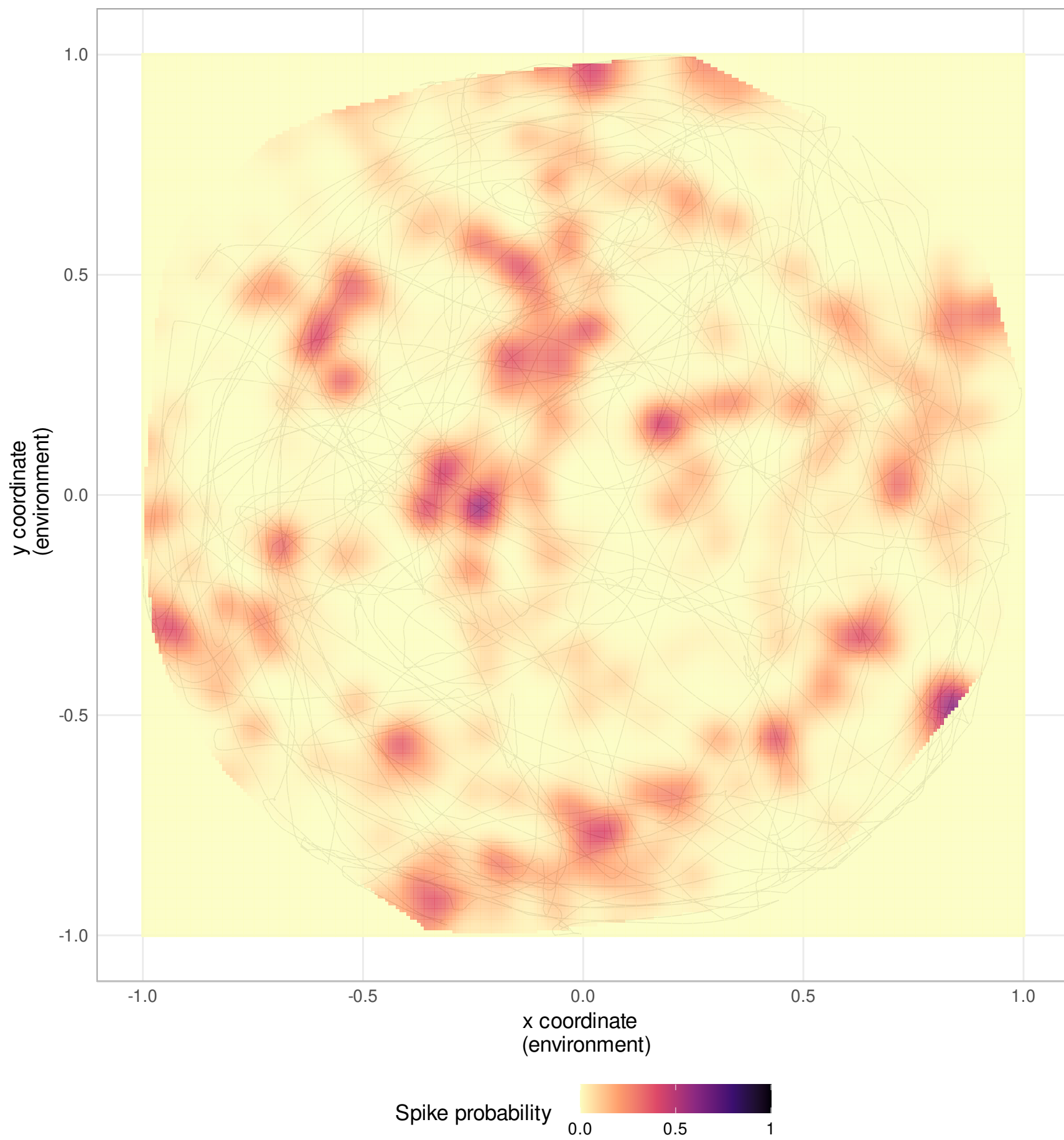
Neuron 172
