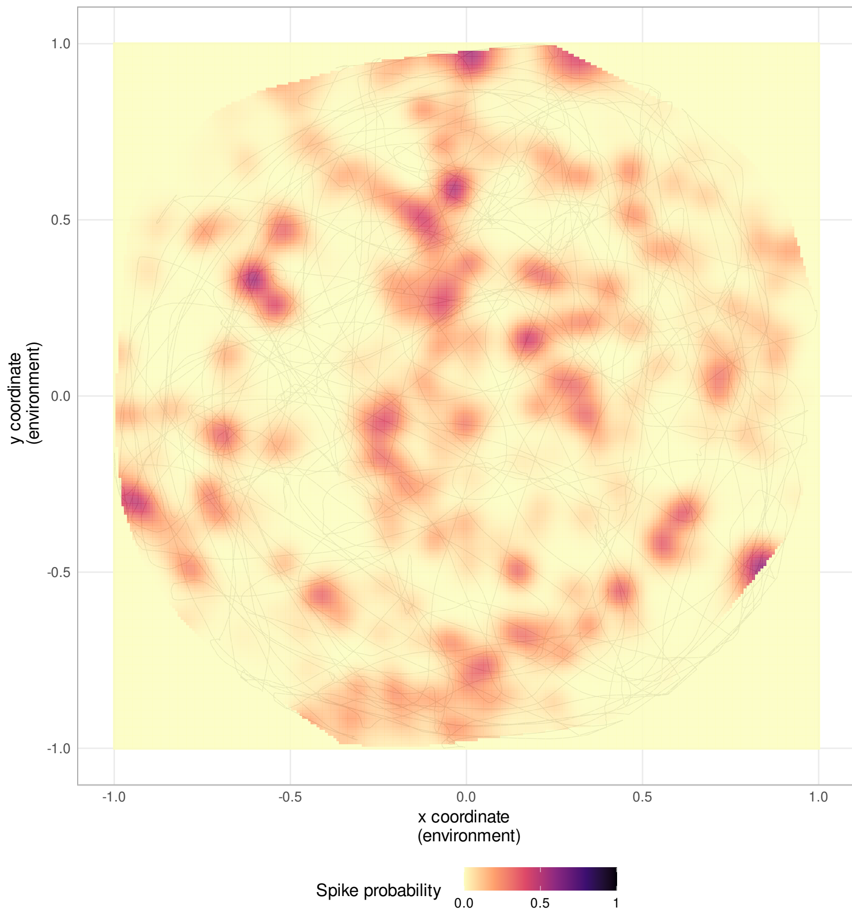
Neuron 175
