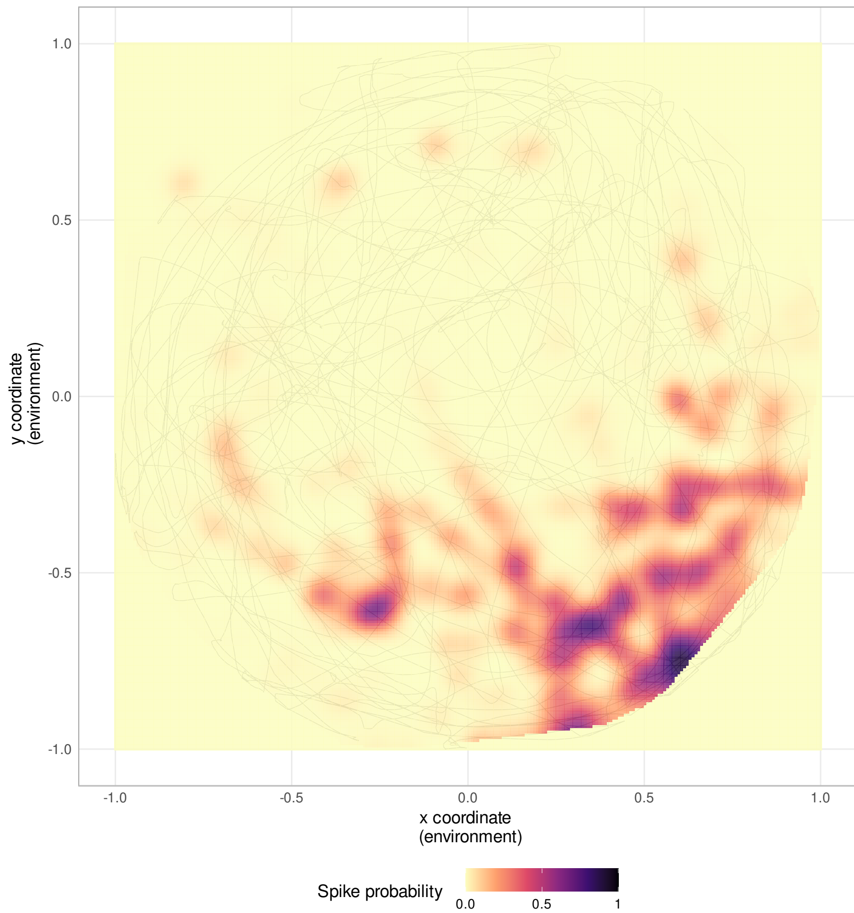
Neuron 182
