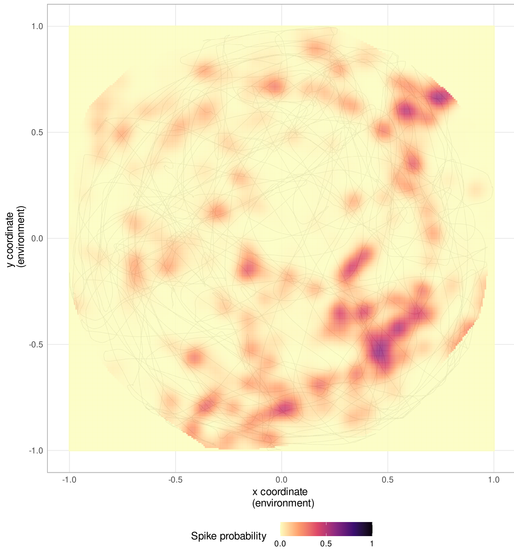
Neuron 190
