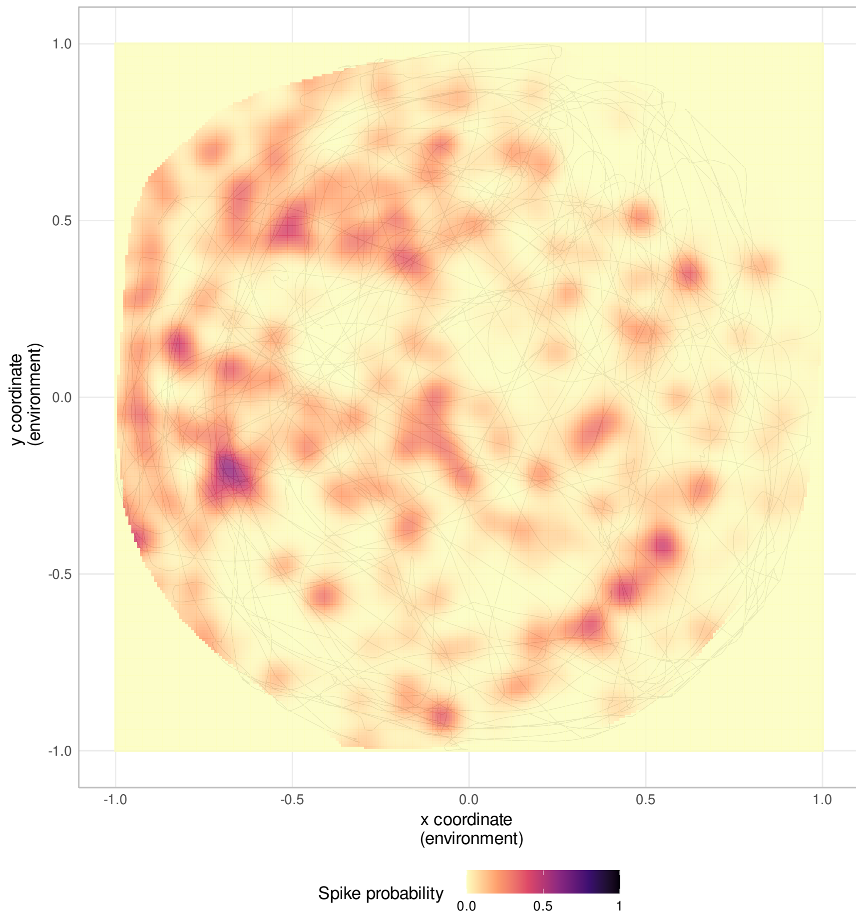
Neuron 193
