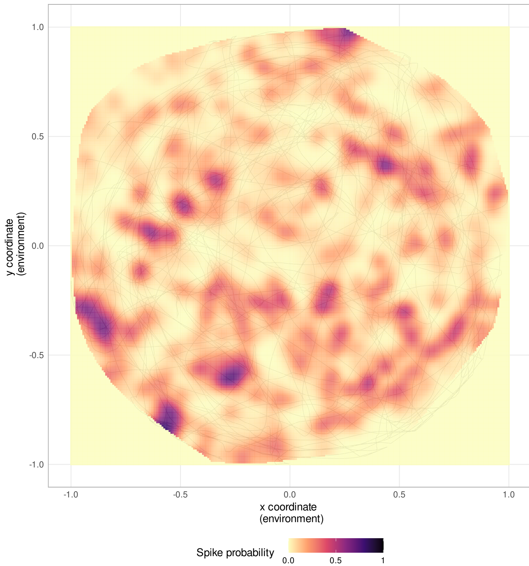
Neuron 2
