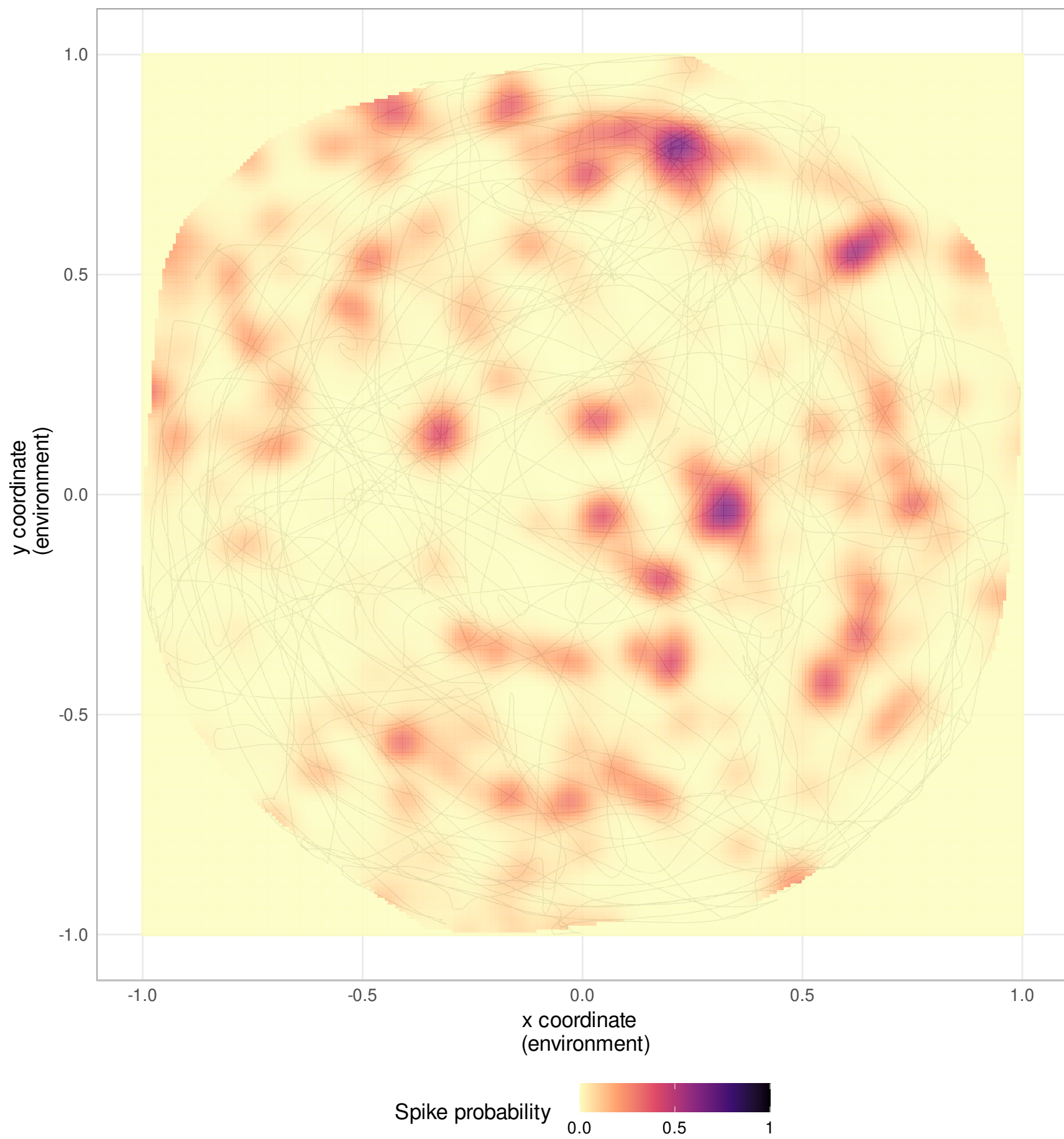
Neuron 21
