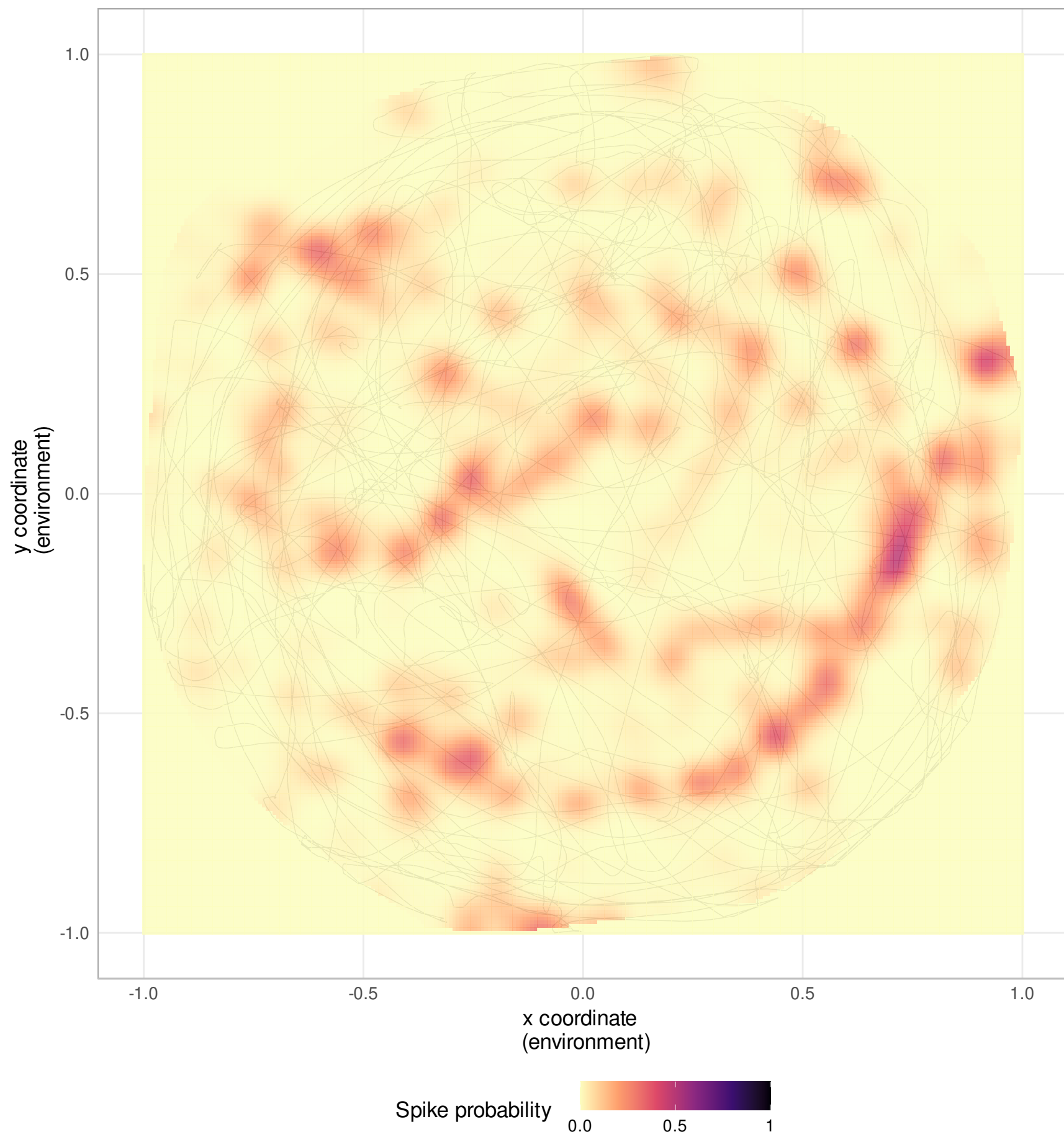
Neuron 210
