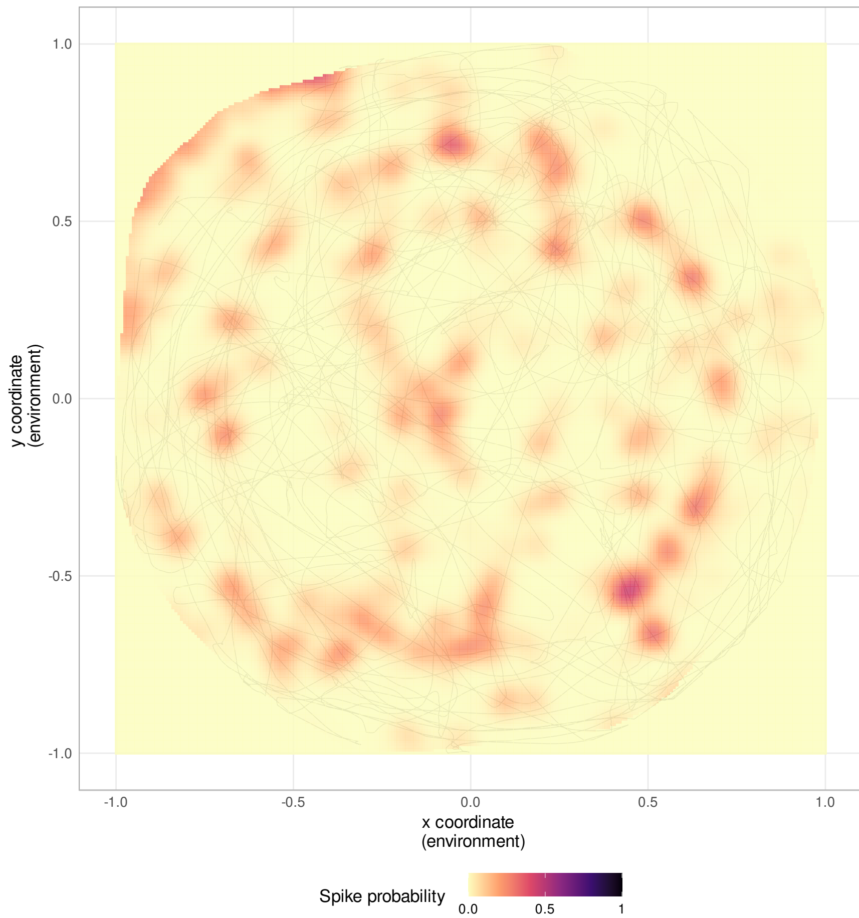
Neuron 216
