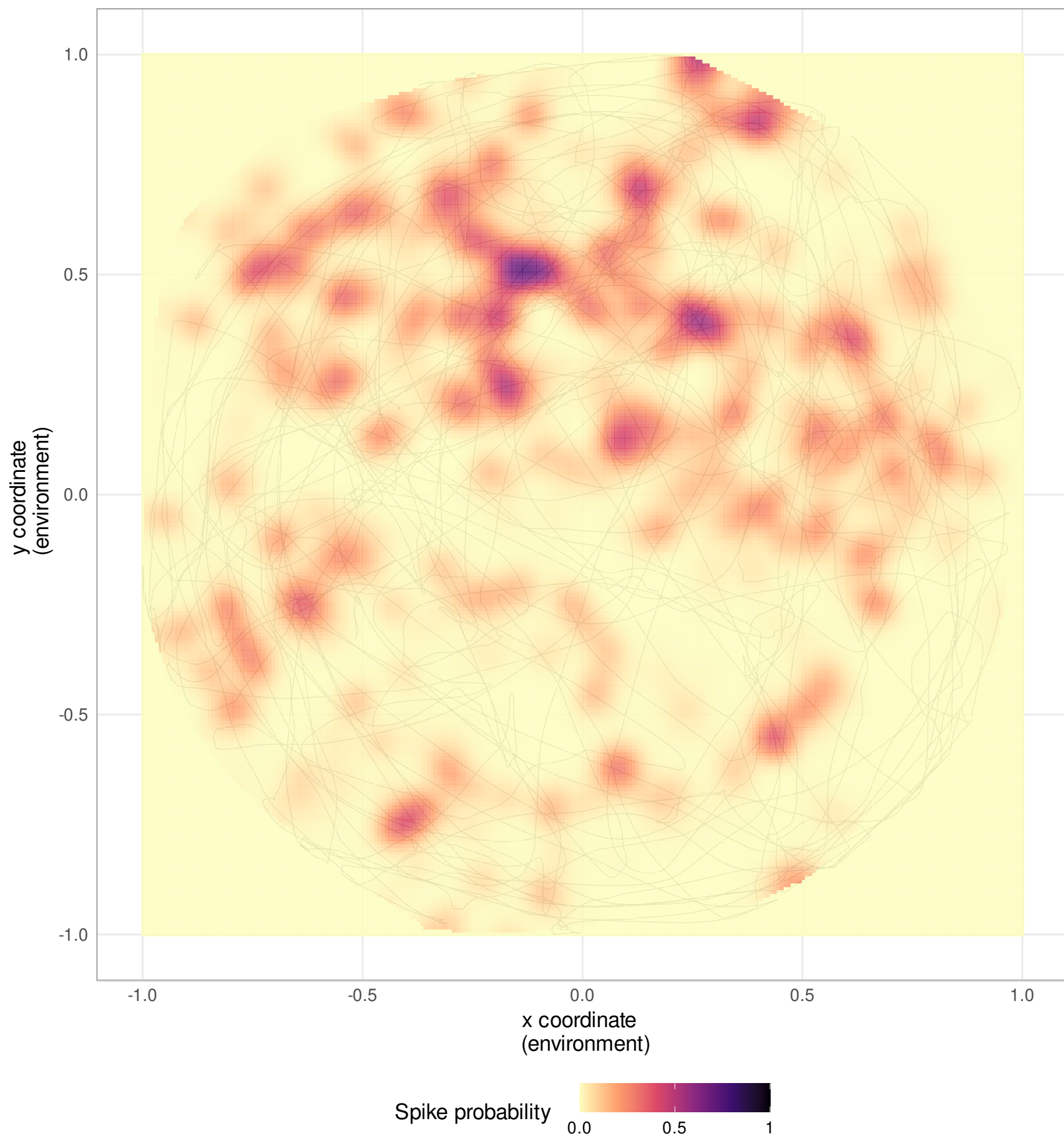
Neuron 22
