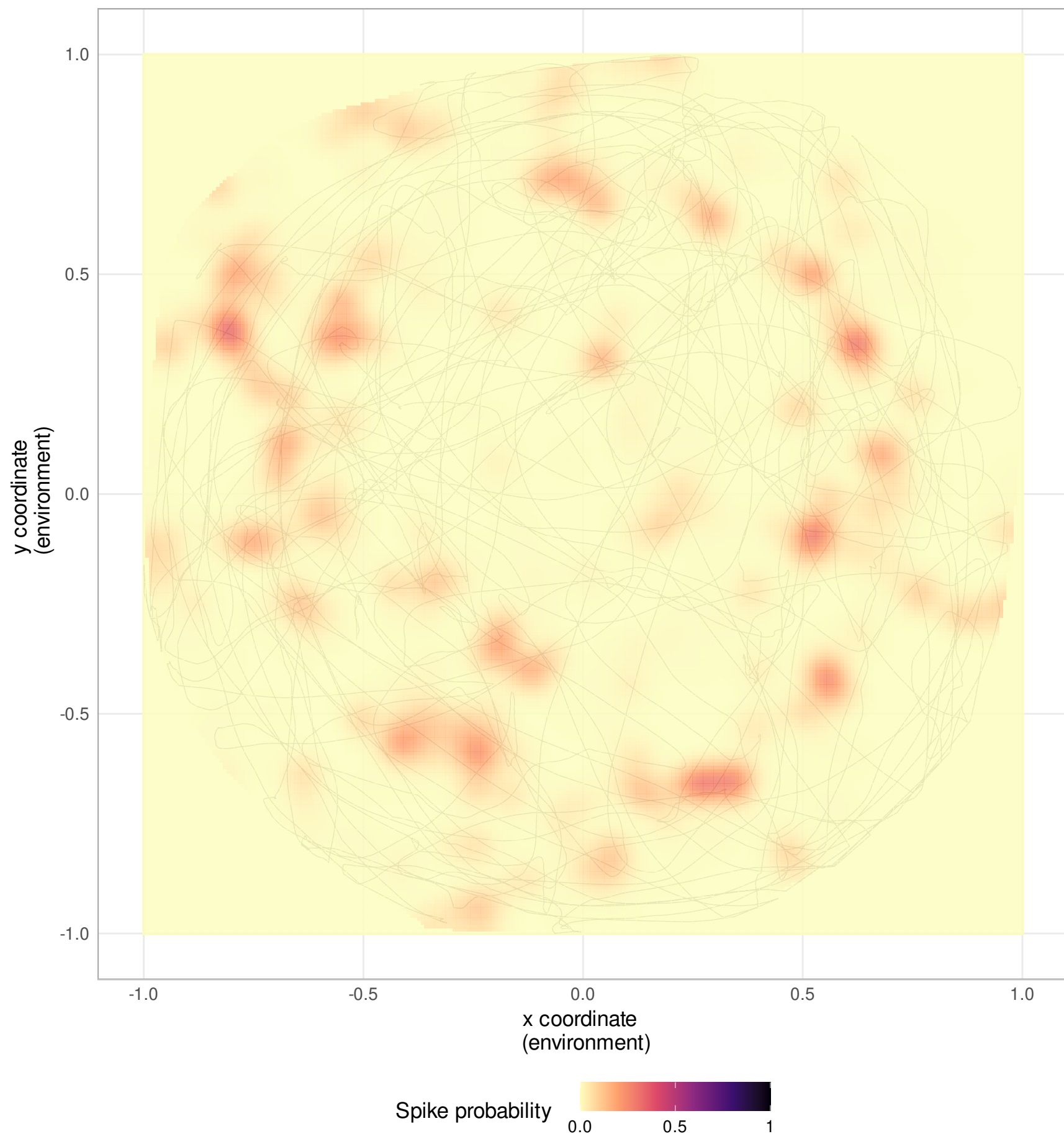
Neuron 230
