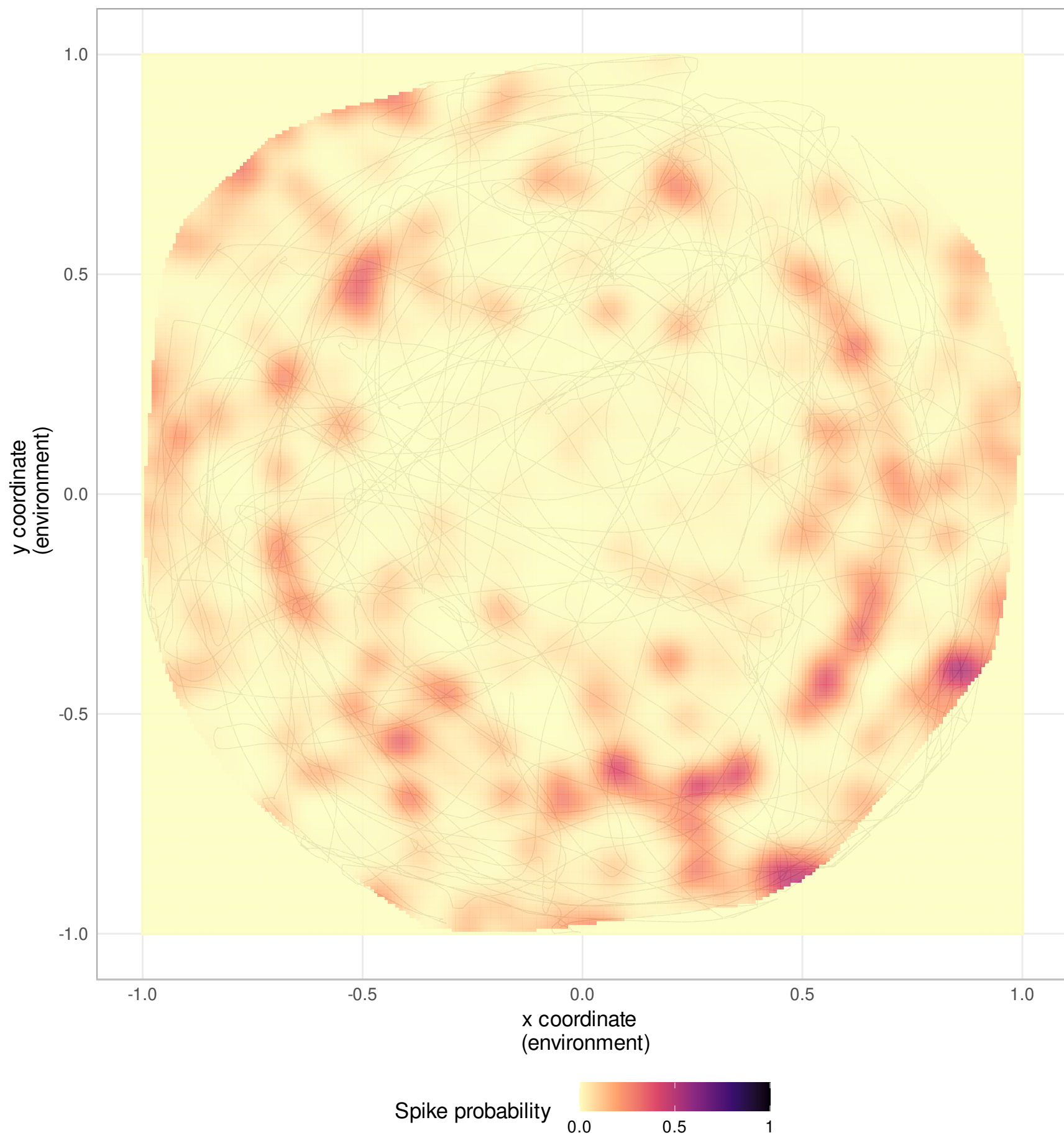
Neuron 232
