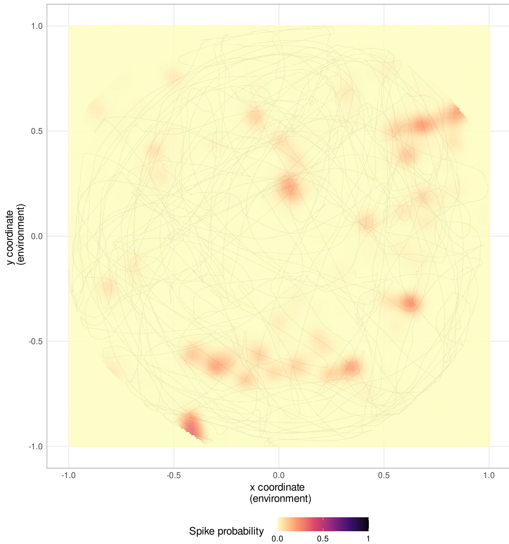
Neuron 233
