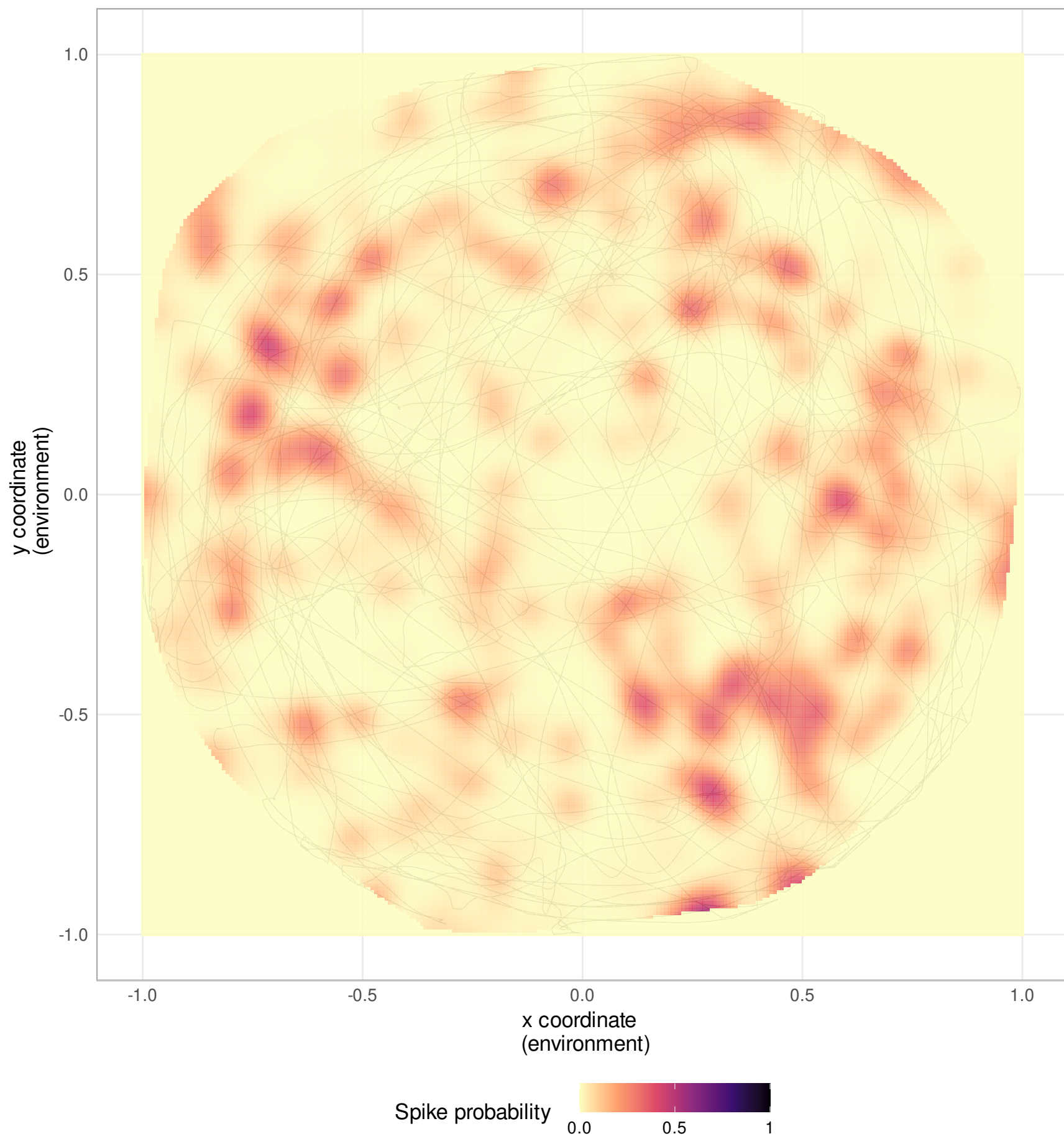
Neuron 234
