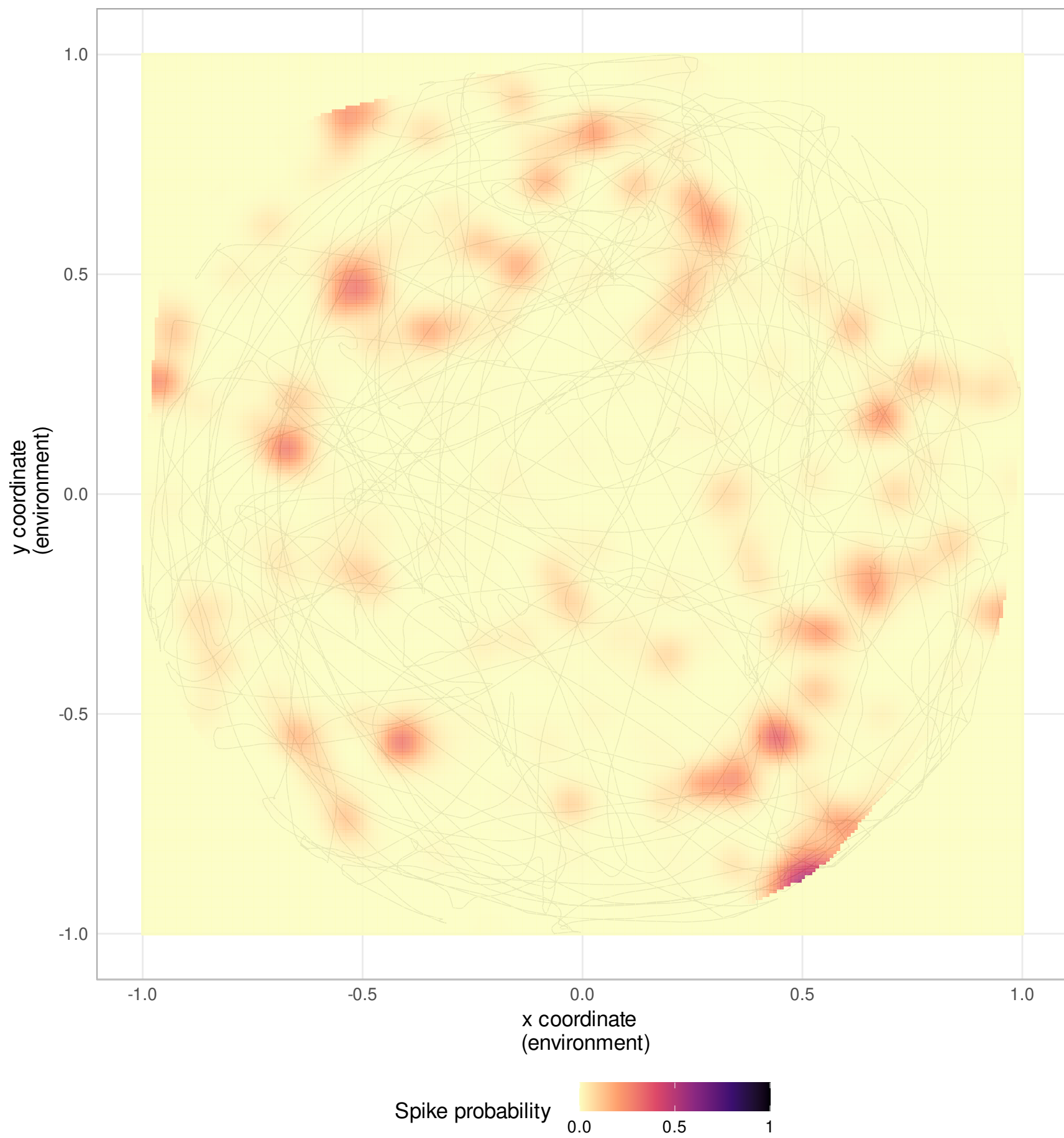
Neuron 235
