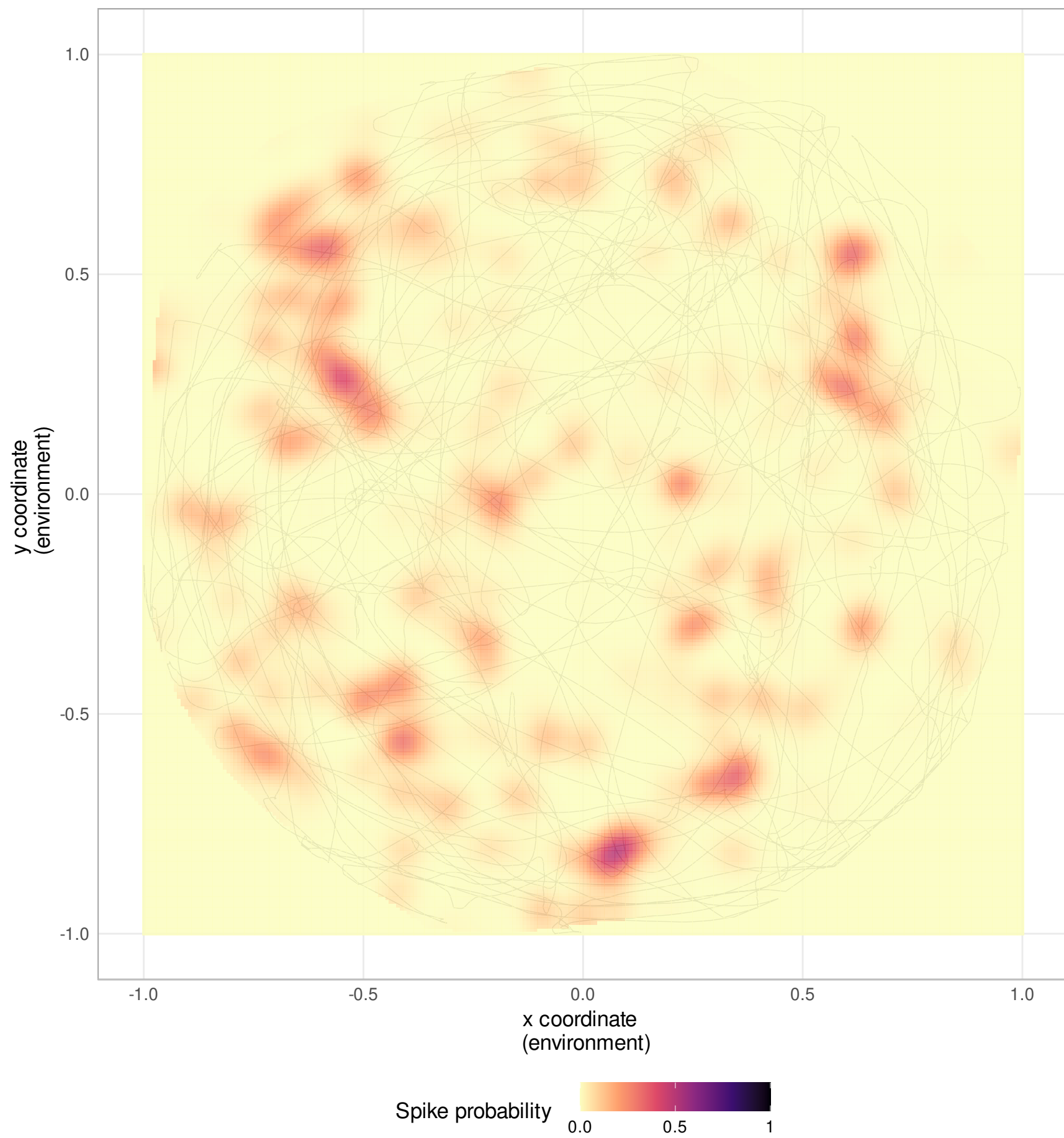
Neuron 249
