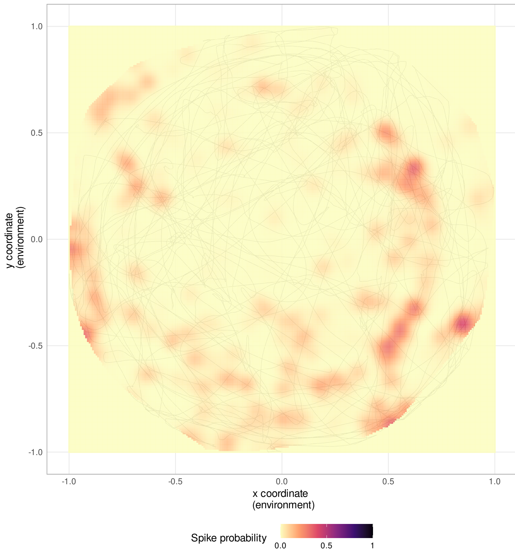
Neuron 250
