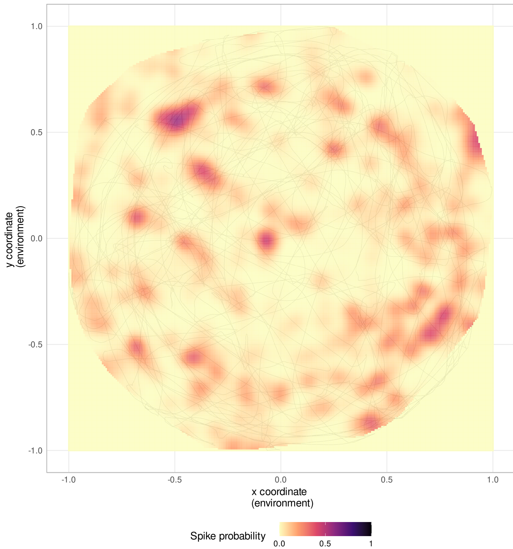
Neuron 252
