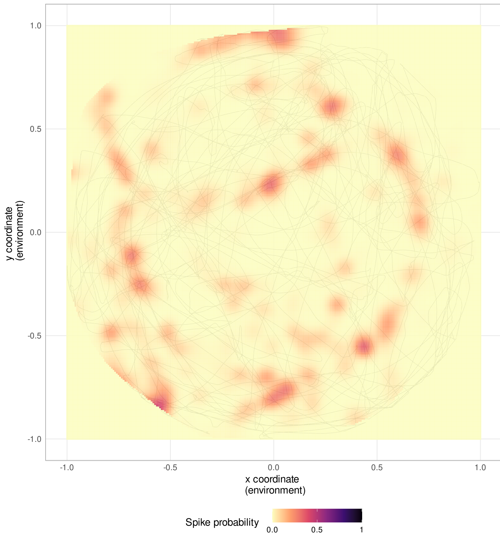
Neuron 253
