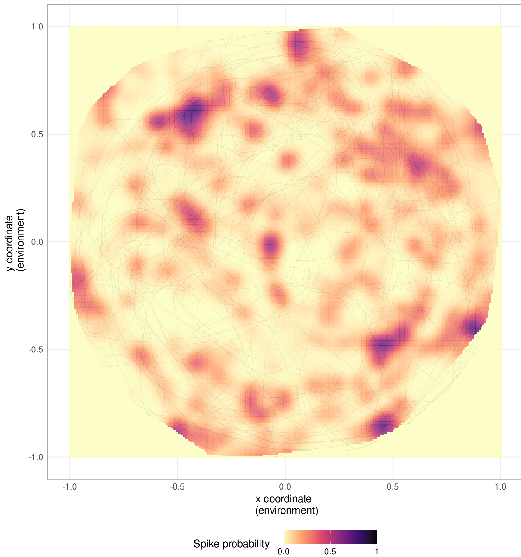
Neuron 26
