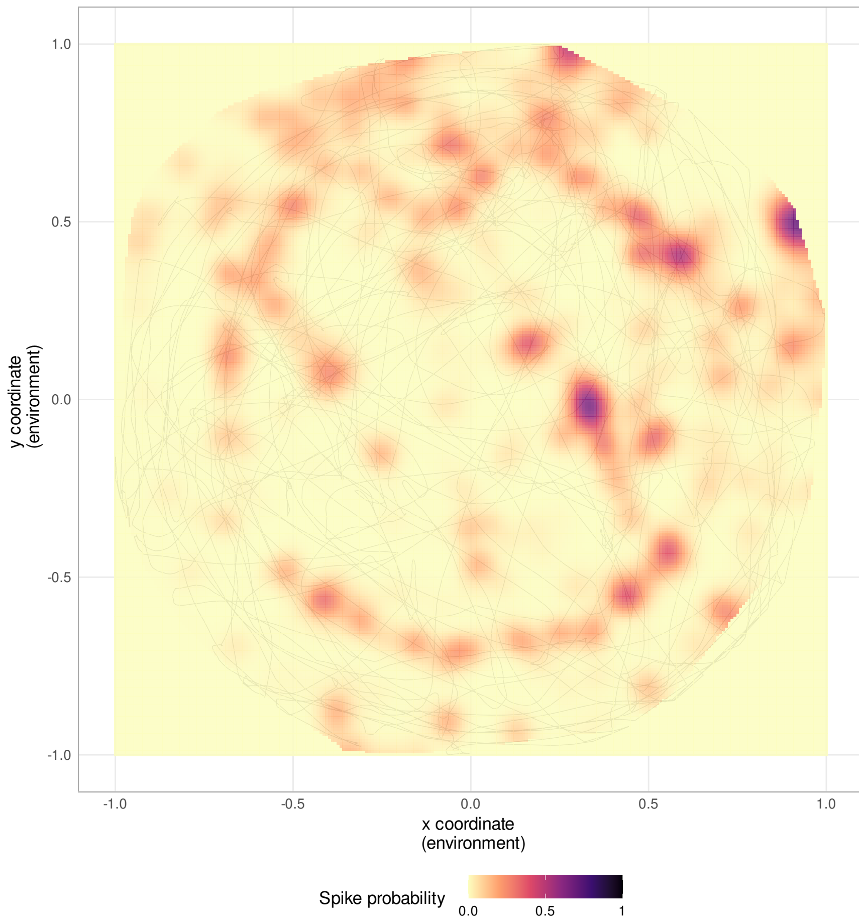
Neuron 267
