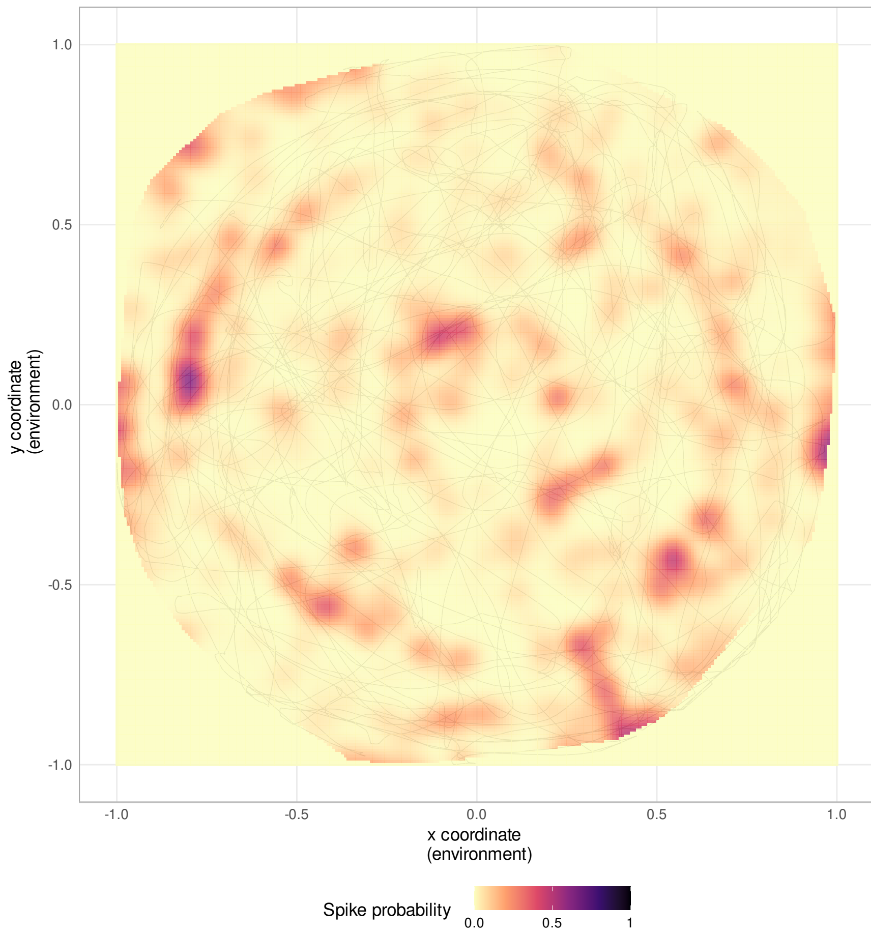
Neuron 27
