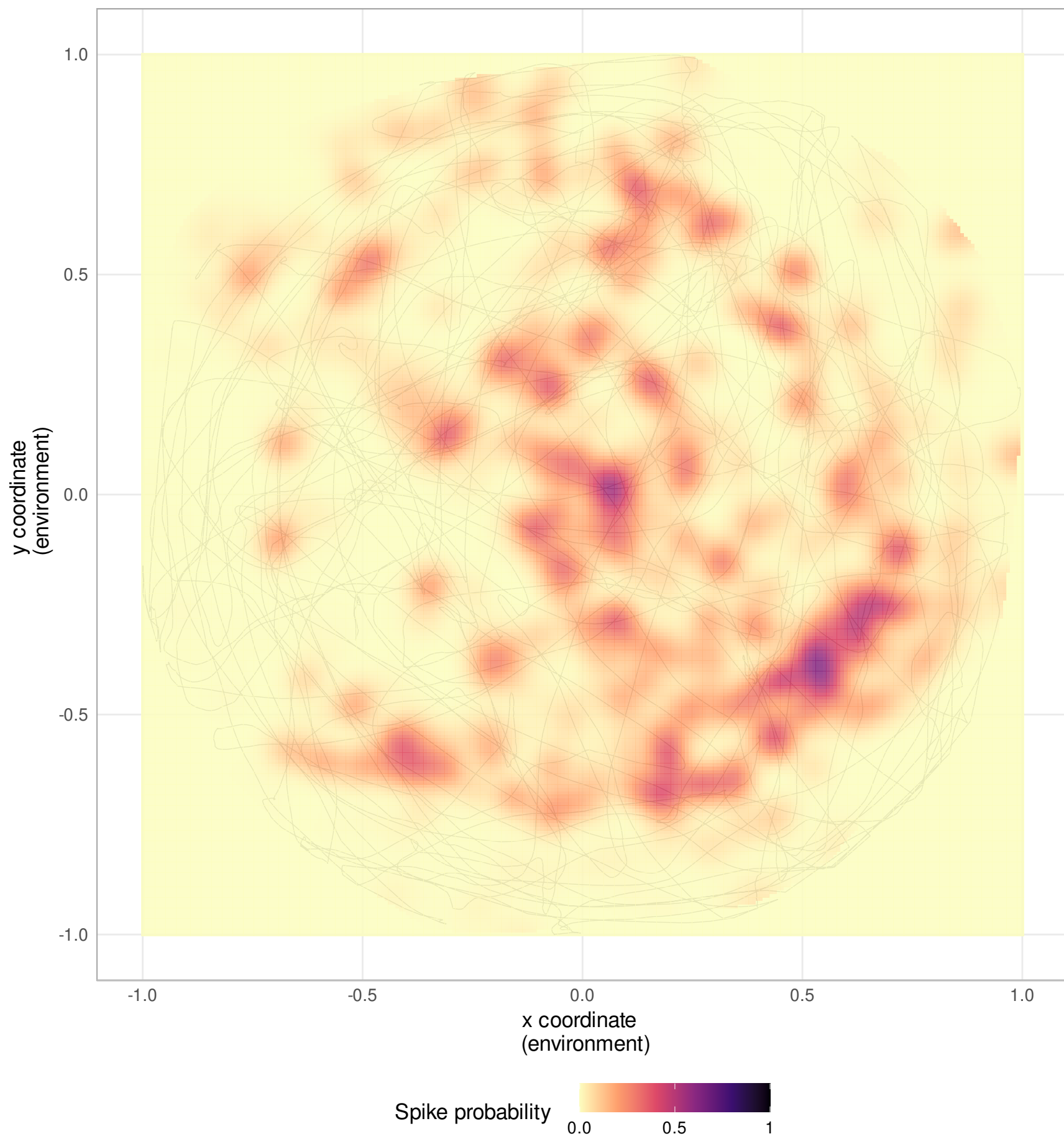
Neuron 276
