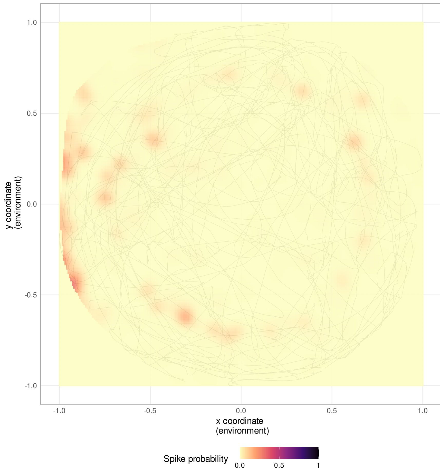
Neuron 280
