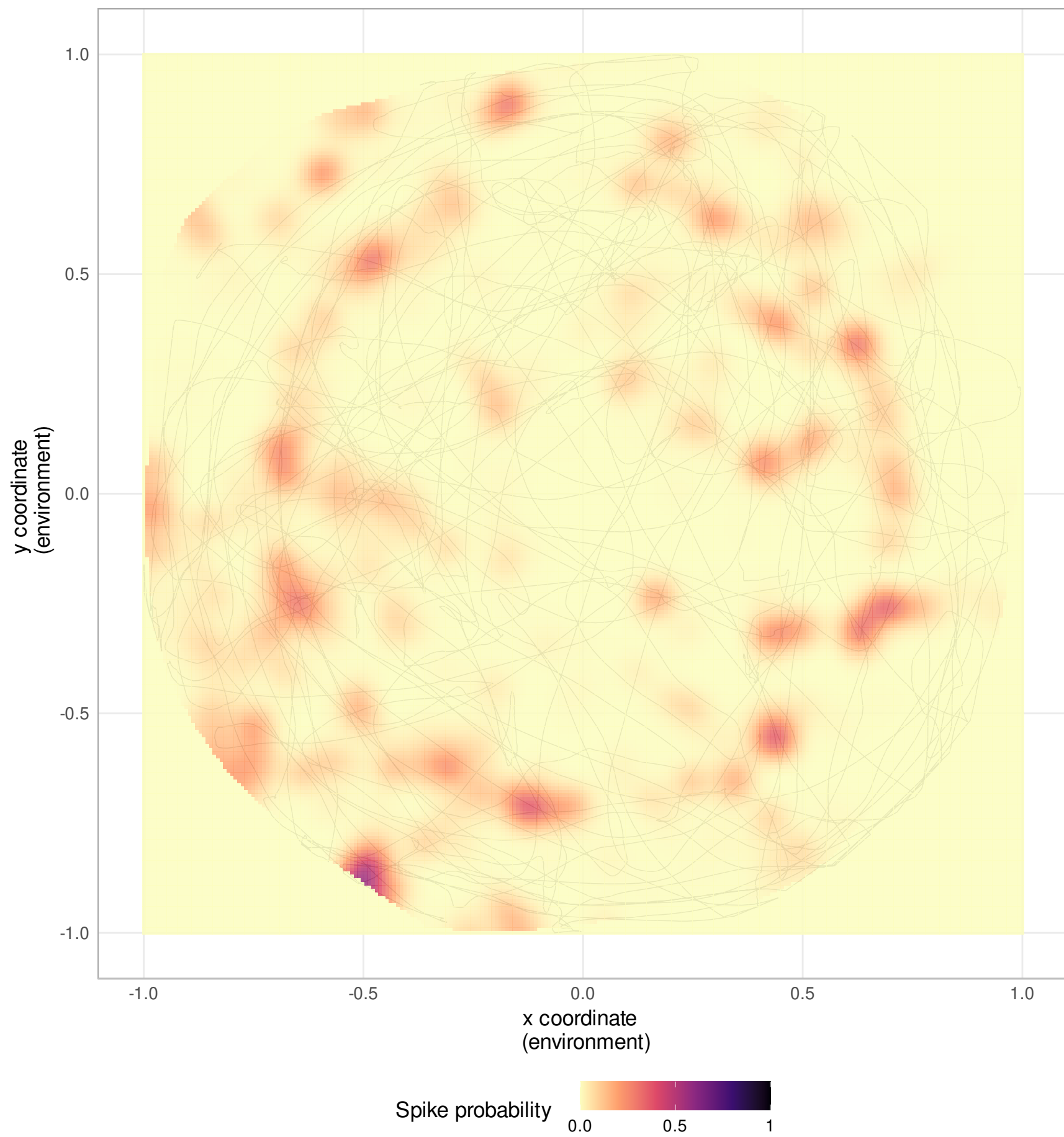
Neuron 287
