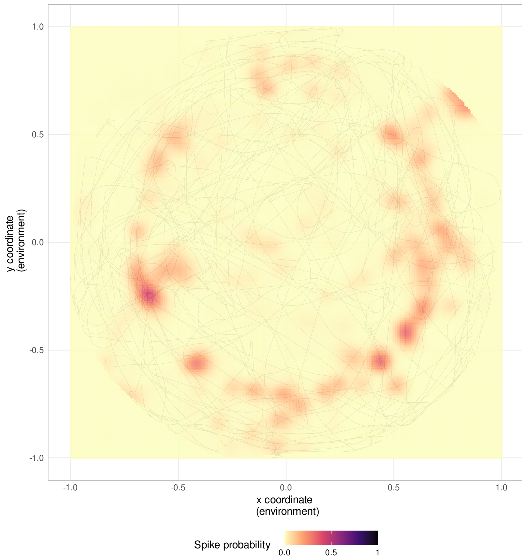
Neuron 319
