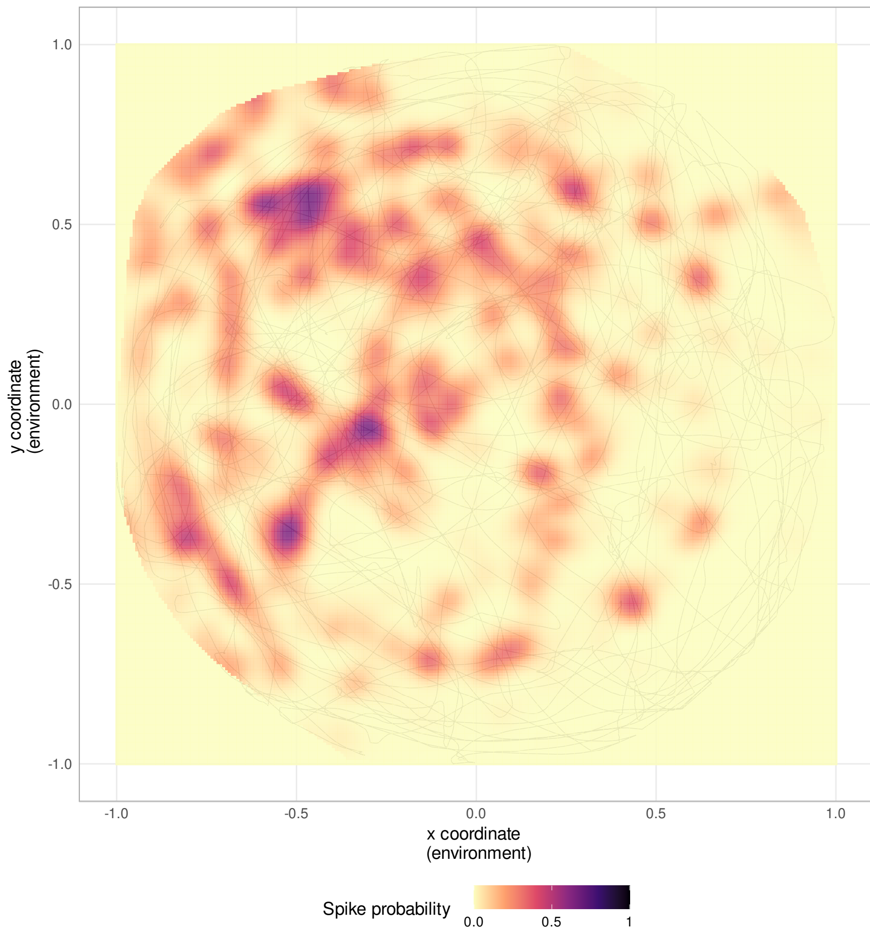
Neuron 35
