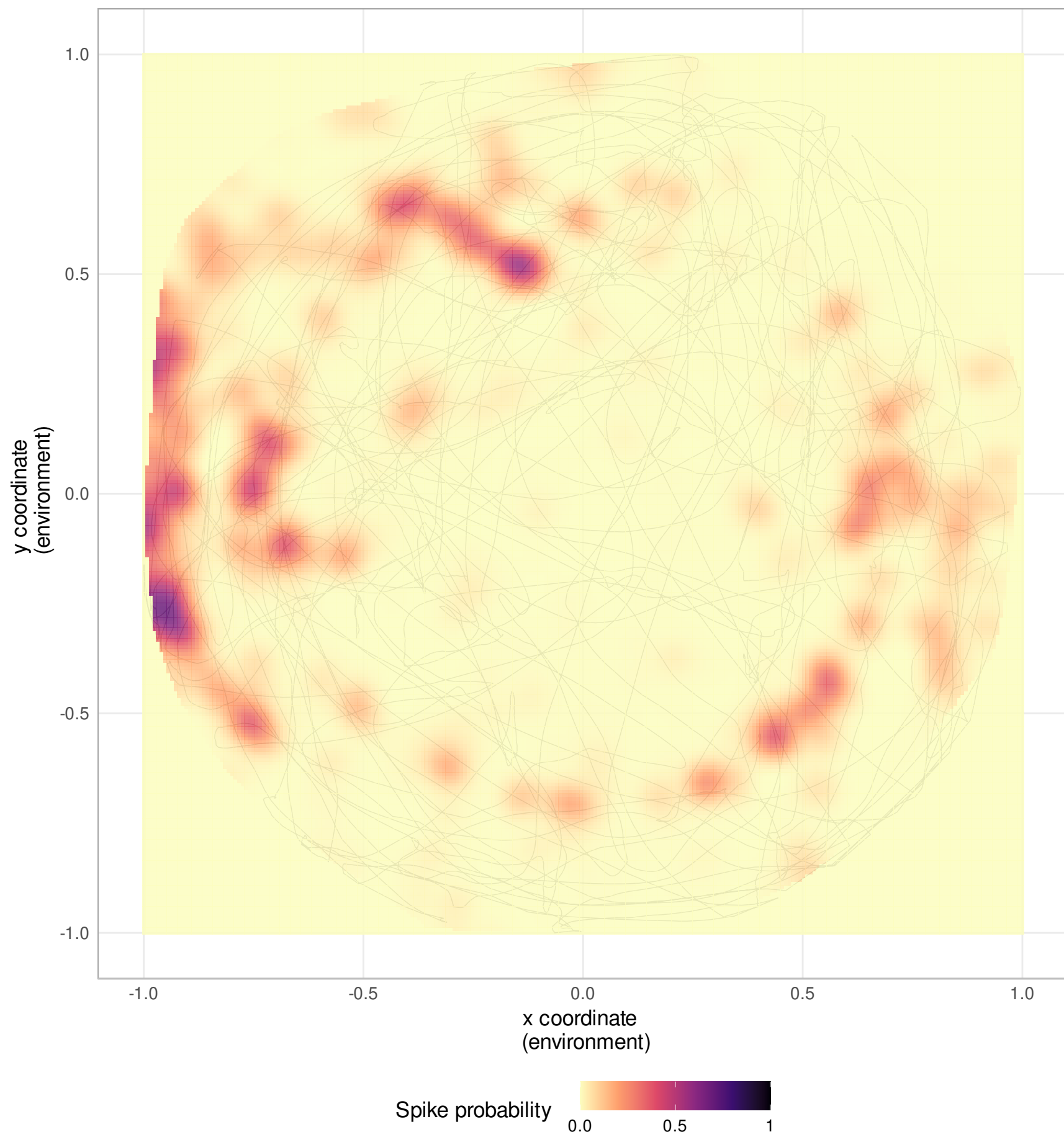
Neuron 53
