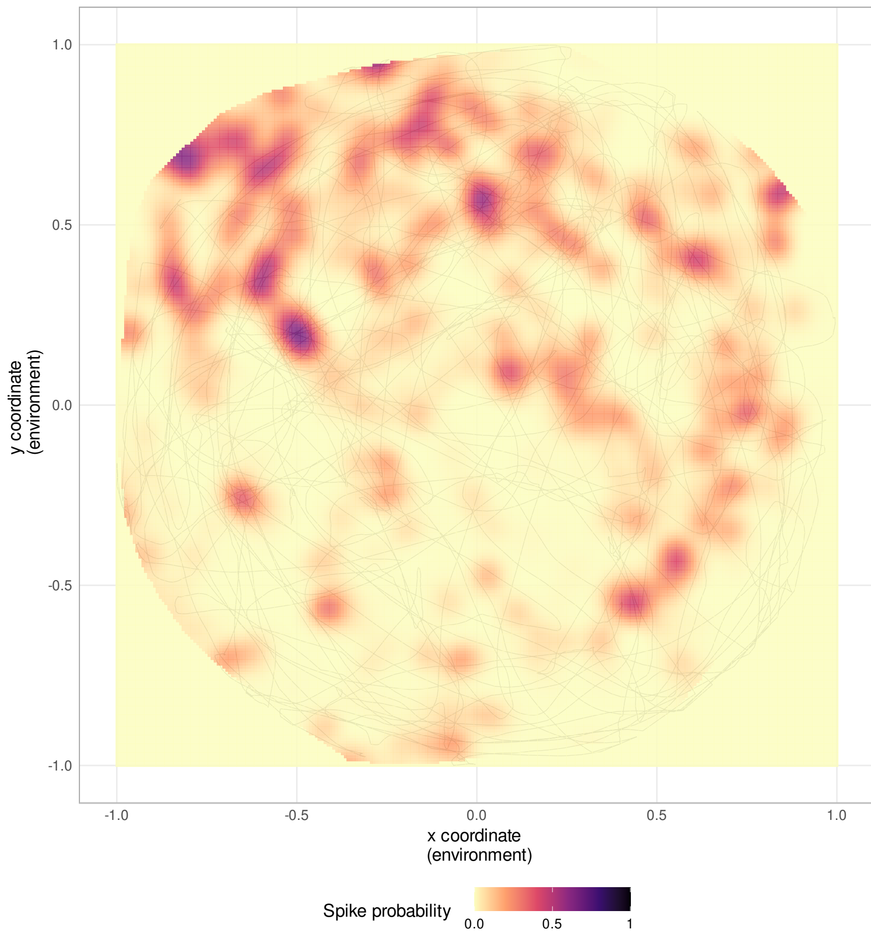
Neuron 55
