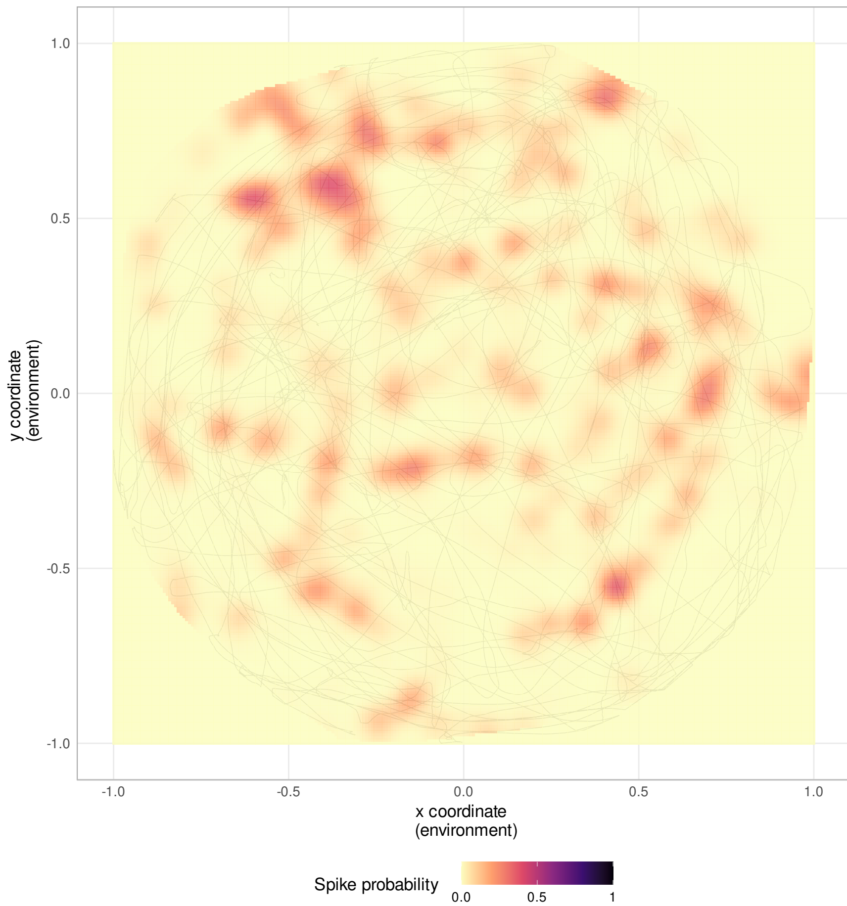
Neuron 62
